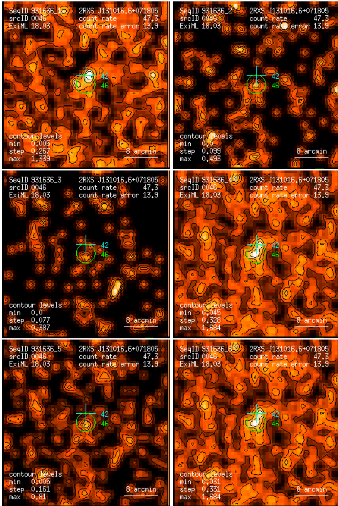
Figure 46: RASS 931636: detection 0046: band rate images, Gaussian filter: (1) PSPC channels 11 – 41, (2) 52 – 90, (3) 91 – 201, (4) 11 – 235, (5) 52 – 201, (6) 11 – 201. Broad band rates in counts/ks. Band rate contour levels in counts/ks/arcmin 2 .
