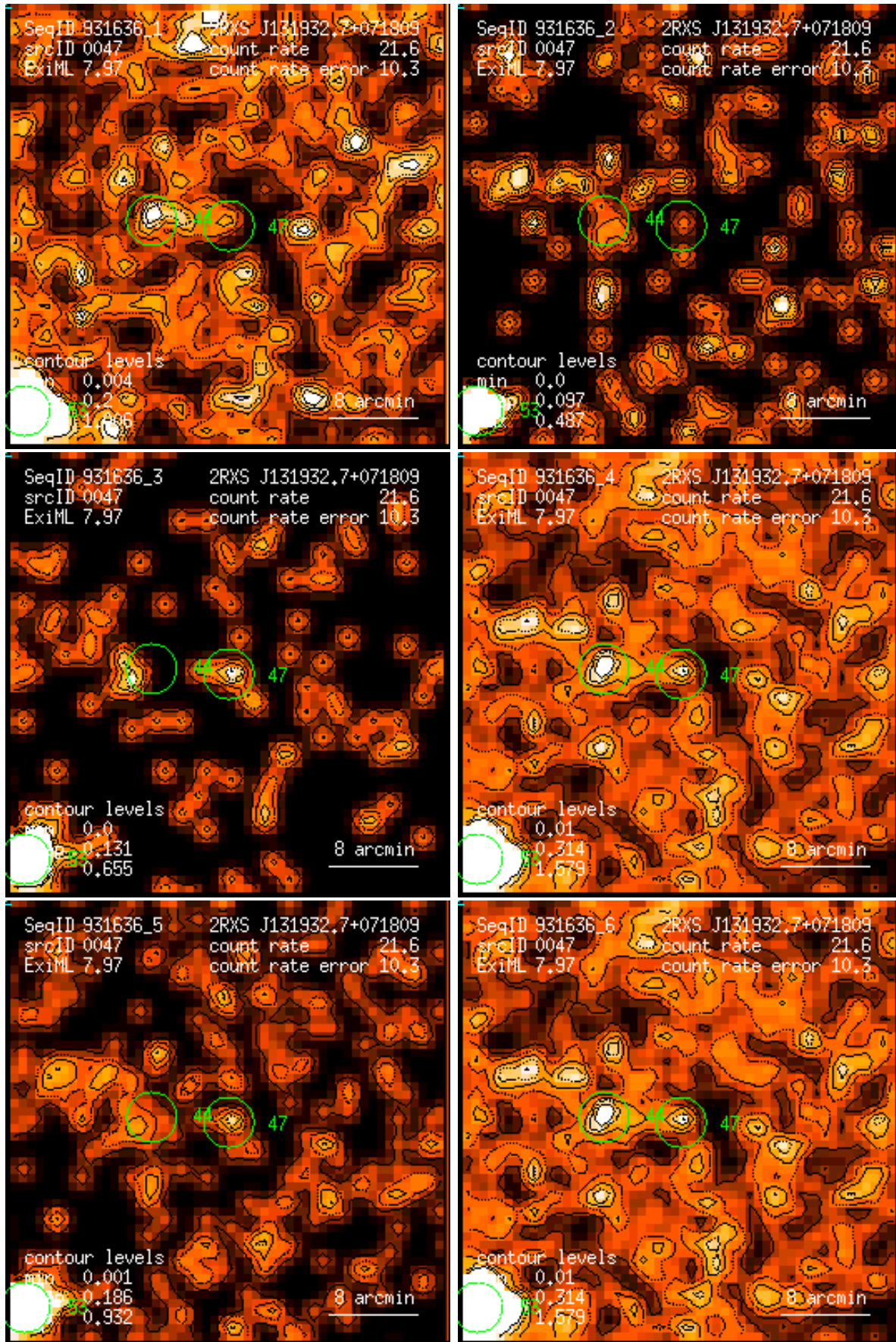
Figure 47: RASS 931636: detection 0047: band rate images, Gaussian filter: (1) PSPC channels 11 – 41, (2) 52 – 90, (3) 91 – 201, (4) 11 – 235, (5) 52 – 201, (6) 11 – 201. Broad band rates in counts/ks. Band rate contour levels in counts/ks/arcmin 2 .
