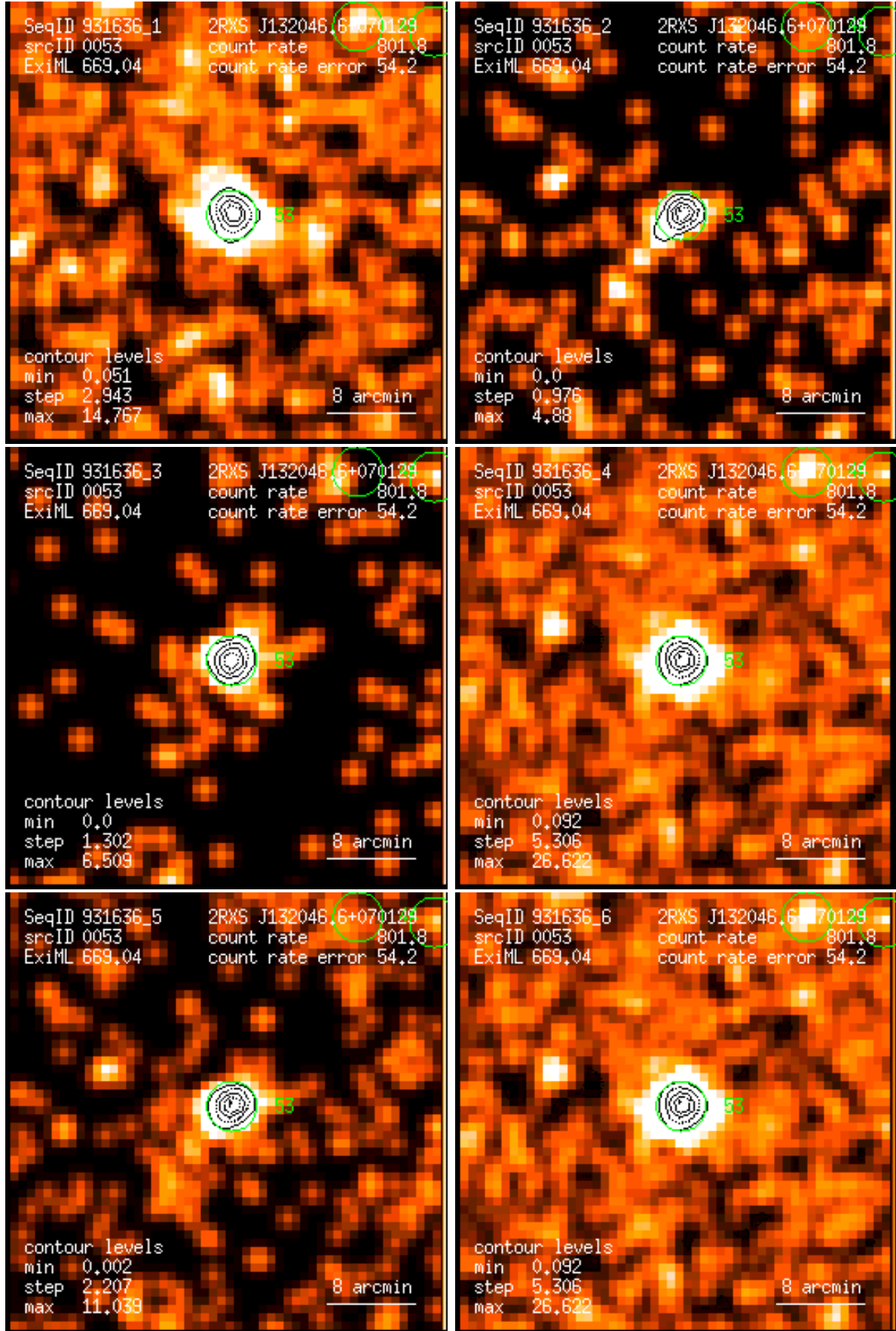
Figure 53: RASS 931636: detection 0053: band rate images, Gaussian filter: (1) PSPC channels 11 – 41, (2) 52 – 90, (3) 91 – 201, (4) 11 – 235, (5) 52 – 201, (6) 11 – 201. Broad band rates in counts/ks. Band rate contour levels in counts/ks/arcmin 2 .
