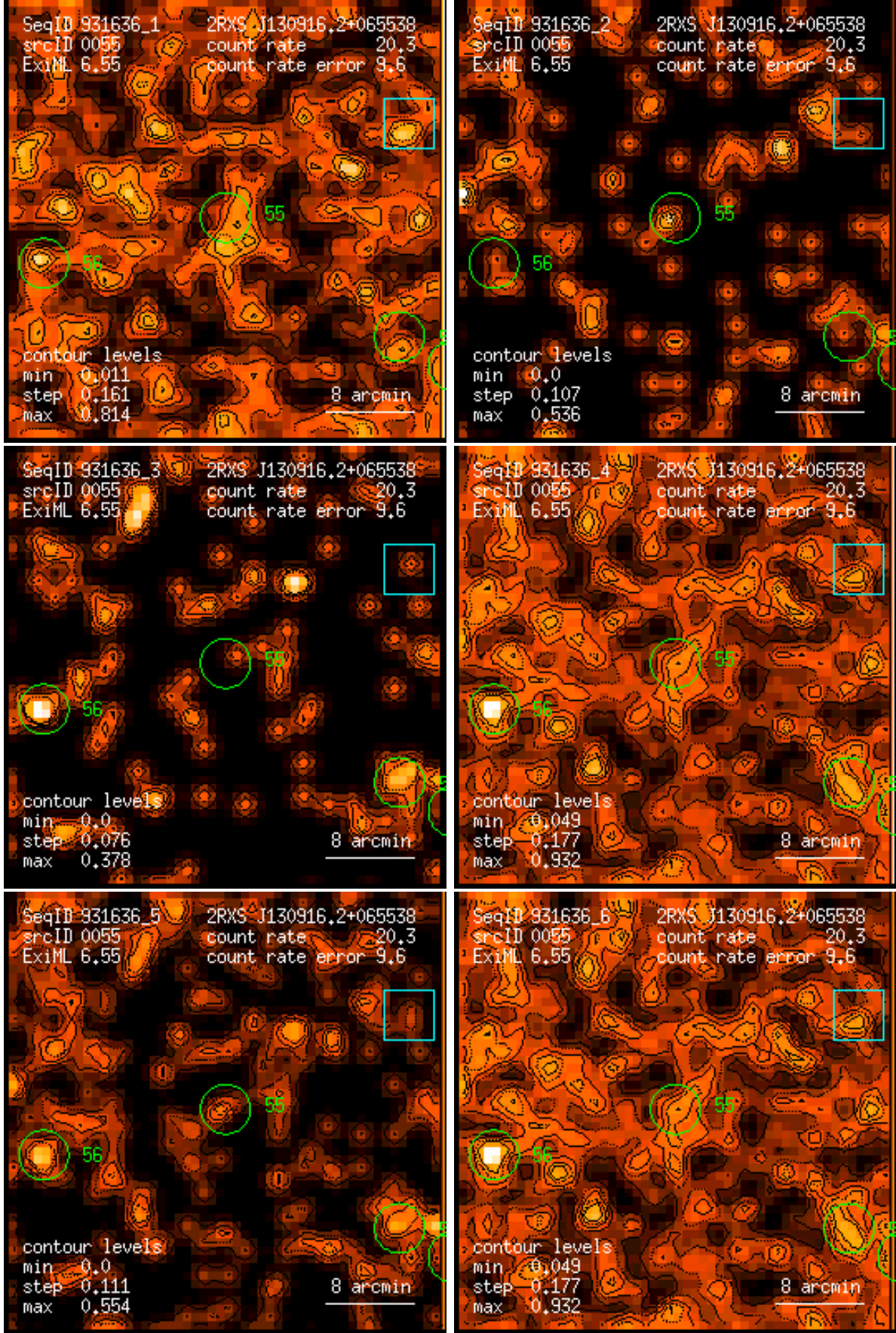
Figure 55: RASS 931636: detection 0055: band rate images, Gaussian filter: (1) PSPC channels 11 – 41, (2) 52 – 90, (3) 91 – 201, (4) 11 – 235, (5) 52 – 201, (6) 11 – 201. Broad band rates in counts/ks. Band rate contour levels in counts/ks/arcmin 2 .
