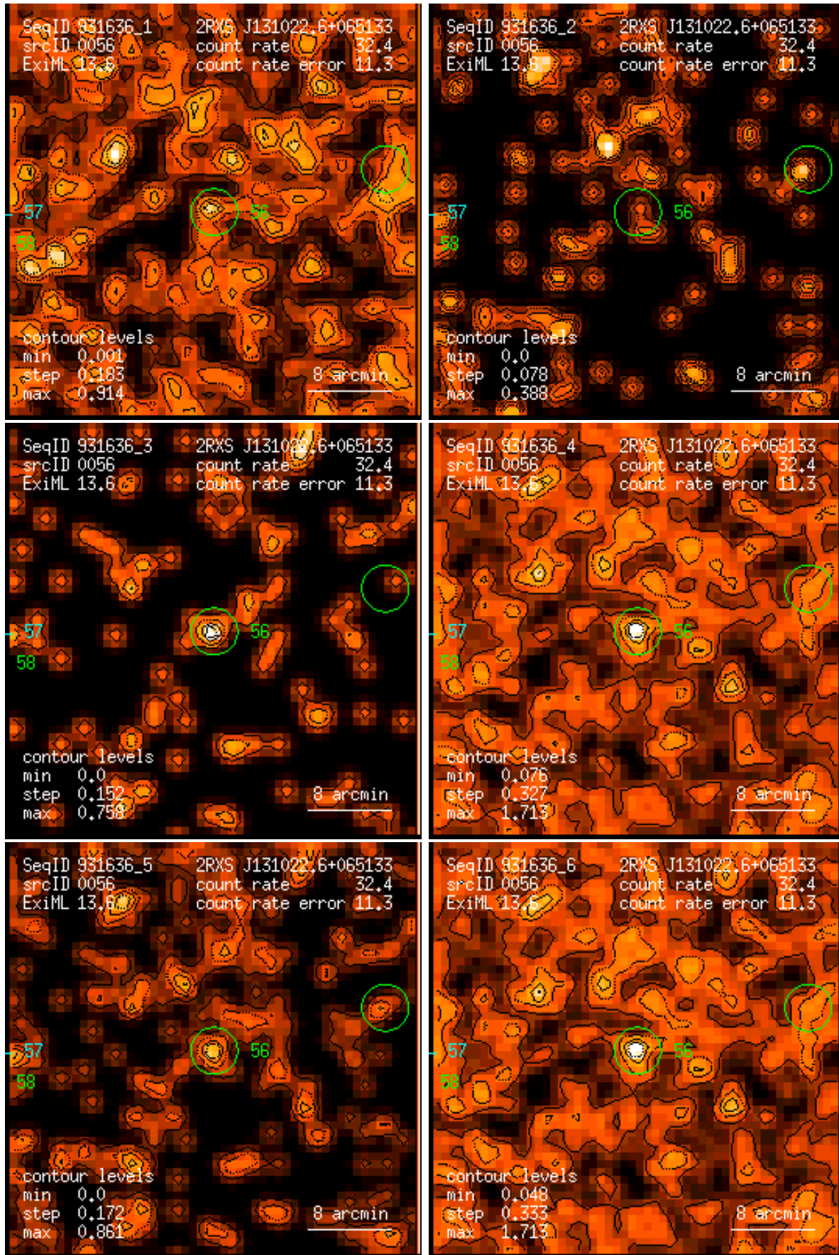
Figure 56: RASS 931636: detection 0056: band rate images, Gaussian filter: (1) PSPC channels 11 – 41, (2) 52 – 90, (3) 91 – 201, (4) 11 – 235, (5) 52 – 201, (6) 11 – 201. Broad band rates in counts/ks. Band rate contour levels in counts/ks/arcmin 2 .
