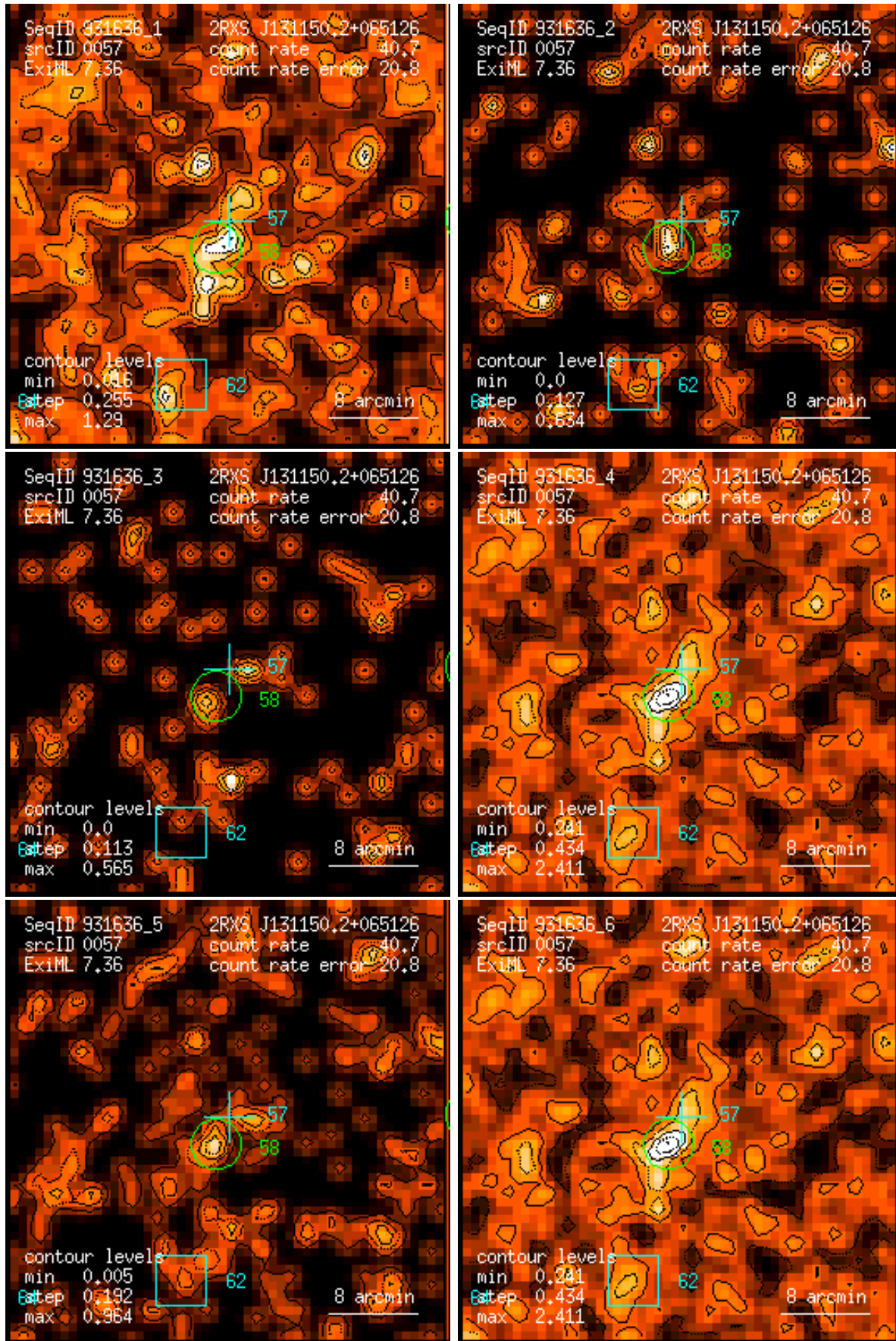
Figure 57: RASS 931636: detection 0057: band rate images, Gaussian filter: (1) PSPC channels 11 – 41, (2) 52 – 90, (3) 91 – 201, (4) 11 – 235, (5) 52 – 201, (6) 11 – 201. Broad band rates in counts/ks. Band rate contour levels in counts/ks/arcmin 2 .
