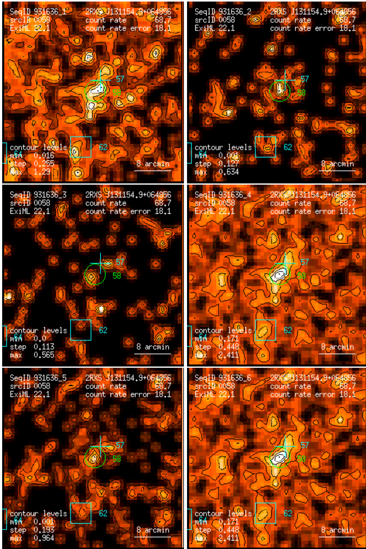
Figure 58: RASS 931636: detection 0058: band rate images, Gaussian filter: (1) PSPC channels 11 – 41, (2) 52 – 90, (3) 91 – 201, (4) 11 – 235, (5) 52 – 201, (6) 11 – 201. Broad band rates in counts/ks. Band rate contour levels in counts/ks/arcmin 2 .
