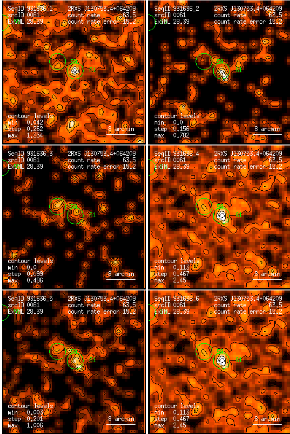
Figure 61: RASS 931636: detection 0061: band rate images, Gaussian filter: (1) PSPC channels 11 – 41, (2) 52 – 90, (3) 91 – 201, (4) 11 – 235, (5) 52 – 201, (6) 11 – 201. Broad band rates in counts/ks. Band rate contour levels in counts/ks/arcmin 2 .
