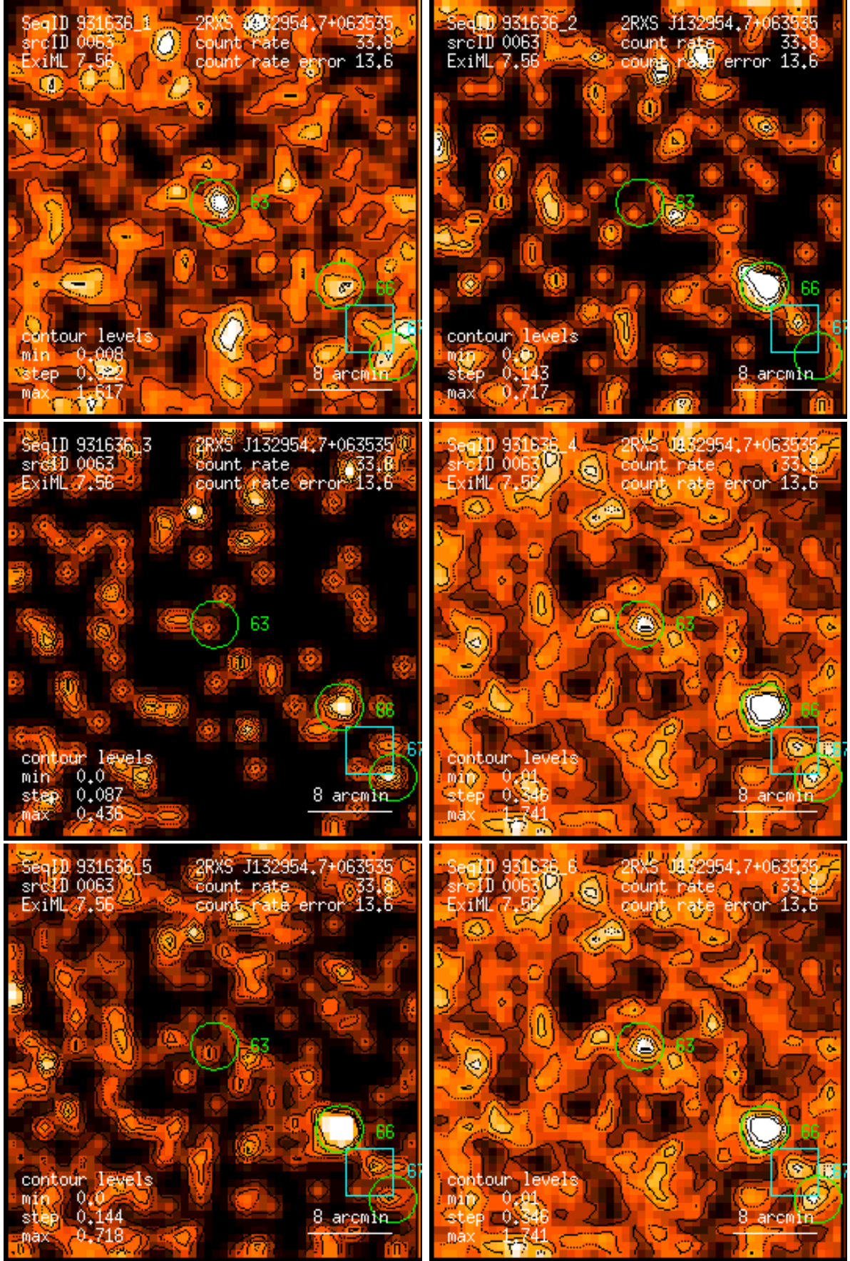
Figure 63: RASS 931636: detection 0063: band rate images, Gaussian filter: (1) PSPC channels 11 – 41, (2) 52 – 90, (3) 91 – 201, (4) 11 – 235, (5) 52 – 201, (6) 11 – 201. Broad band rates in counts/ks. Band rate contour levels in counts/ks/arcmin 2 .
