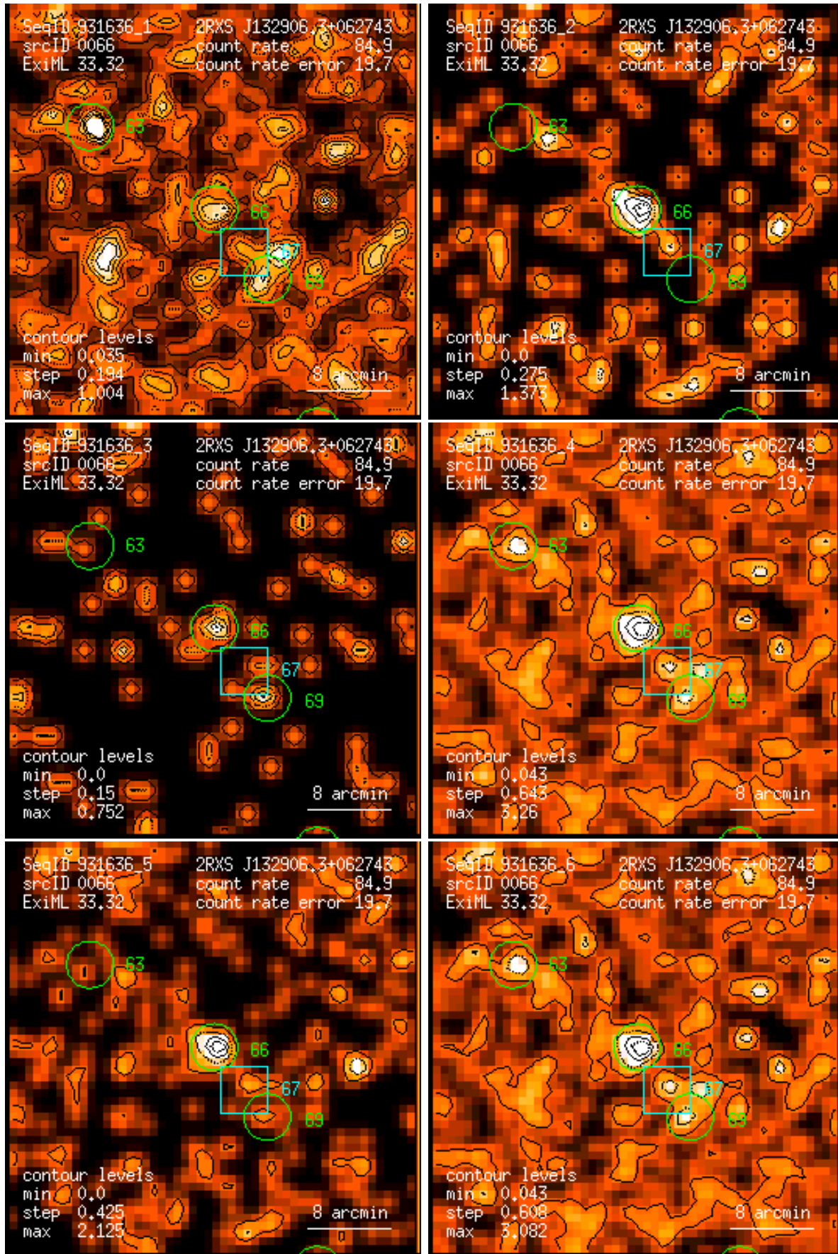
Figure 66: RASS 931636: detection 0066: band rate images, Gaussian filter: (1) PSPC channels 11 – 41, (2) 52 – 90, (3) 91 – 201, (4) 11 – 235, (5) 52 – 201, (6) 11 – 201. Broad band rates in counts/ks. Band rate contour levels in counts/ks/arcmin 2 .
