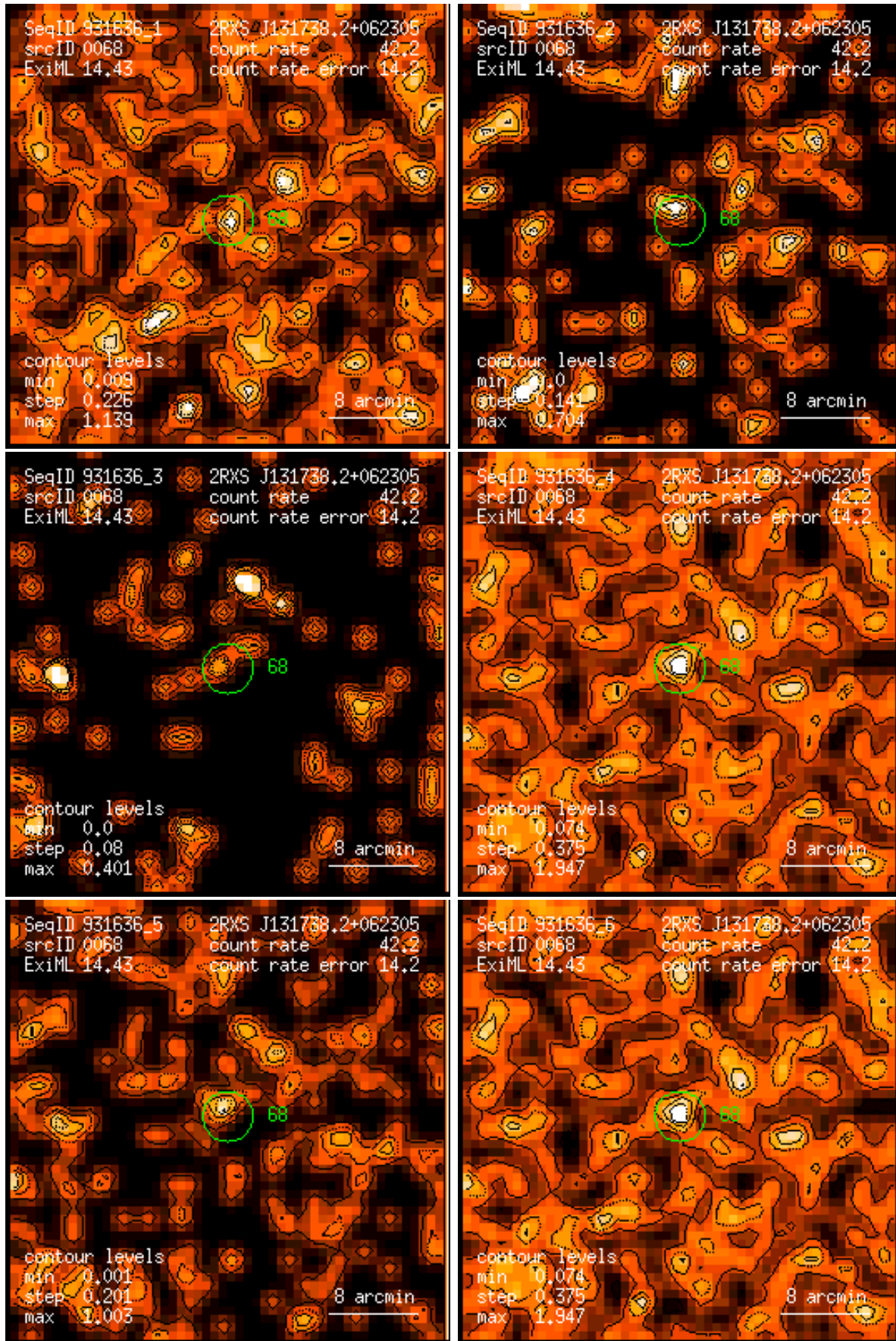
Figure 68: RASS 931636: detection 0068: band rate images, Gaussian filter: (1) PSPC channels 11 – 41, (2) 52 – 90, (3) 91 – 201, (4) 11 – 235, (5) 52 – 201, (6) 11 – 201. Broad band rates in counts/ks. Band rate contour levels in counts/ks/arcmin 2 .
