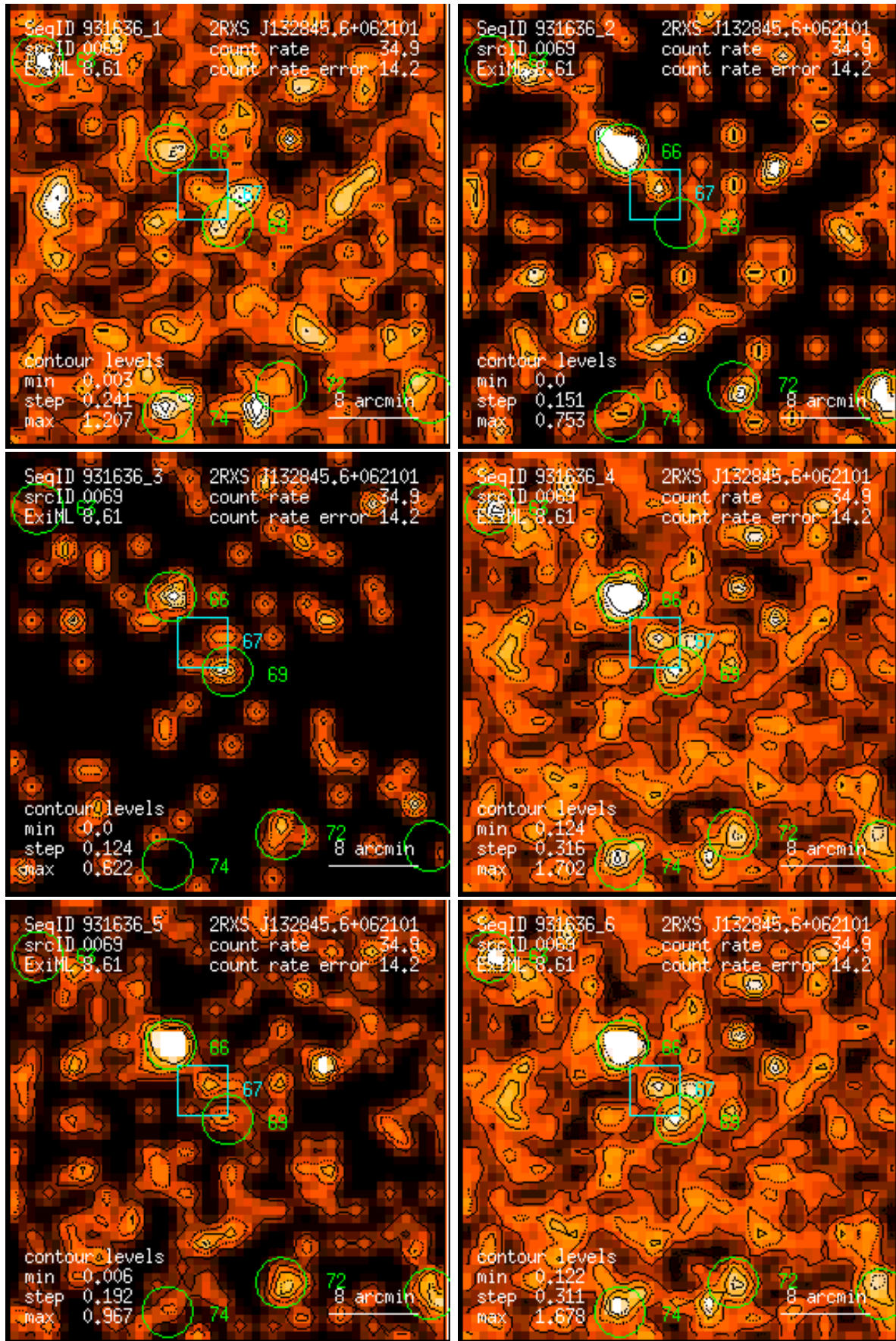
Figure 69: RASS 931636: detection 0069: band rate images, Gaussian filter: (1) PSPC channels 11 – 41, (2) 52 – 90, (3) 91 – 201, (4) 11 – 235, (5) 52 – 201, (6) 11 – 201. Broad band rates in counts/ks. Band rate contour levels in counts/ks/arcmin 2 .
