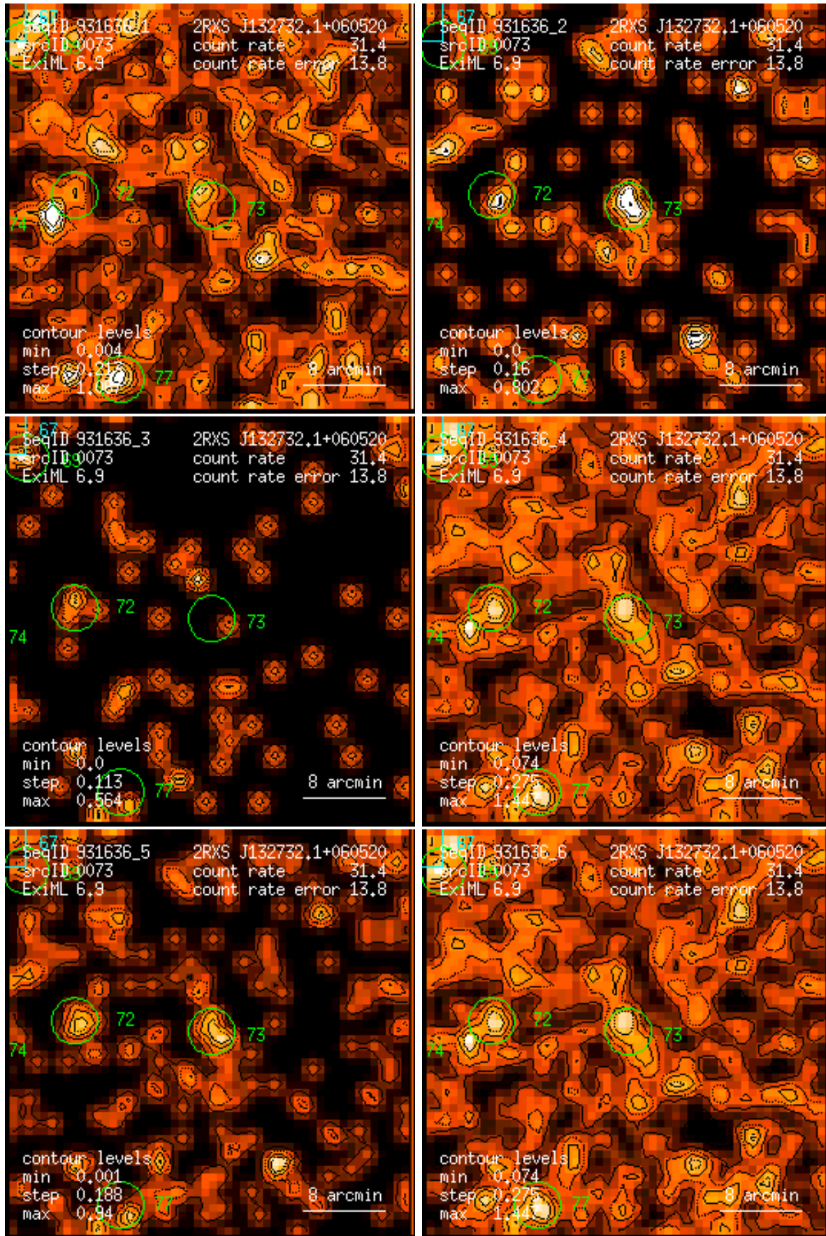
Figure 73: RASS 931636: detection 0073: band rate images, Gaussian filter: (1) PSPC channels 11 – 41, (2) 52 – 90, (3) 91 – 201, (4) 11 – 235, (5) 52 – 201, (6) 11 – 201. Broad band rates in counts/ks. Band rate contour levels in counts/ks/arcmin 2 .
