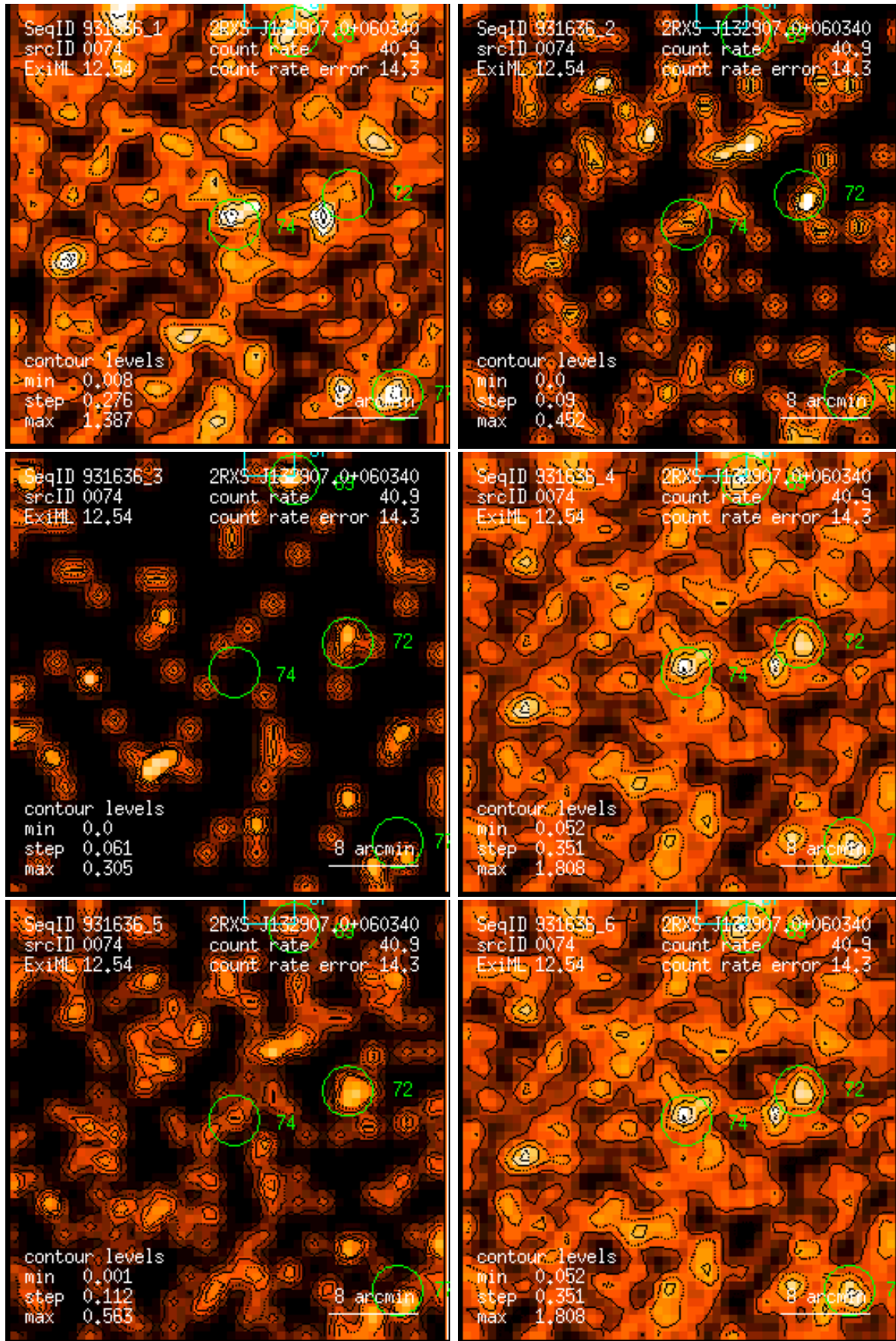
Figure 74: RASS 931636: detection 0074: band rate images, Gaussian filter: (1) PSPC channels 11 – 41, (2) 52 – 90, (3) 91 – 201, (4) 11 – 235, (5) 52 – 201, (6) 11 – 201. Broad band rates in counts/ks. Band rate contour levels in counts/ks/arcmin 2 .
