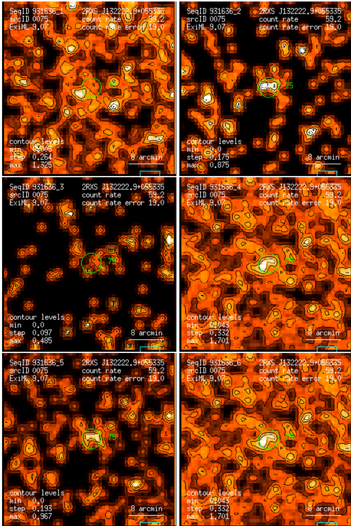
Figure 75: RASS 931636: detection 0075: band rate images, Gaussian filter: (1) PSPC channels 11 – 41, (2) 52 – 90, (3) 91 – 201, (4) 11 – 235, (5) 52 – 201, (6) 11 – 201. Broad band rates in counts/ks. Band rate contour levels in counts/ks/arcmin 2 .
