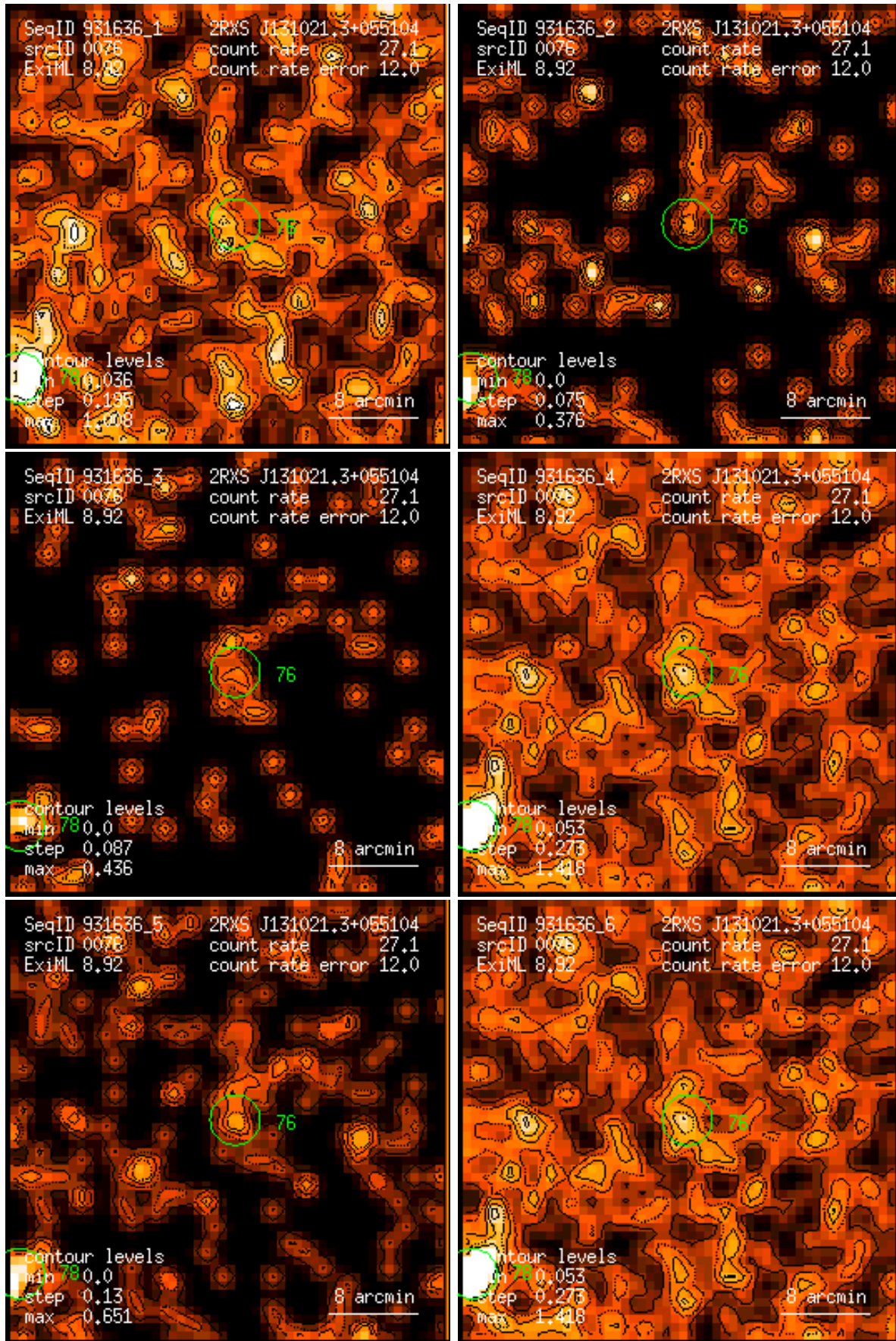
Figure 76: RASS 931636: detection 0076: band rate images, Gaussian filter: (1) PSPC channels 11 – 41, (2) 52 – 90, (3) 91 – 201, (4) 11 – 235, (5) 52 – 201, (6) 11 – 201. Broad band rates in counts/ks. Band rate contour levels in counts/ks/arcmin 2 .
