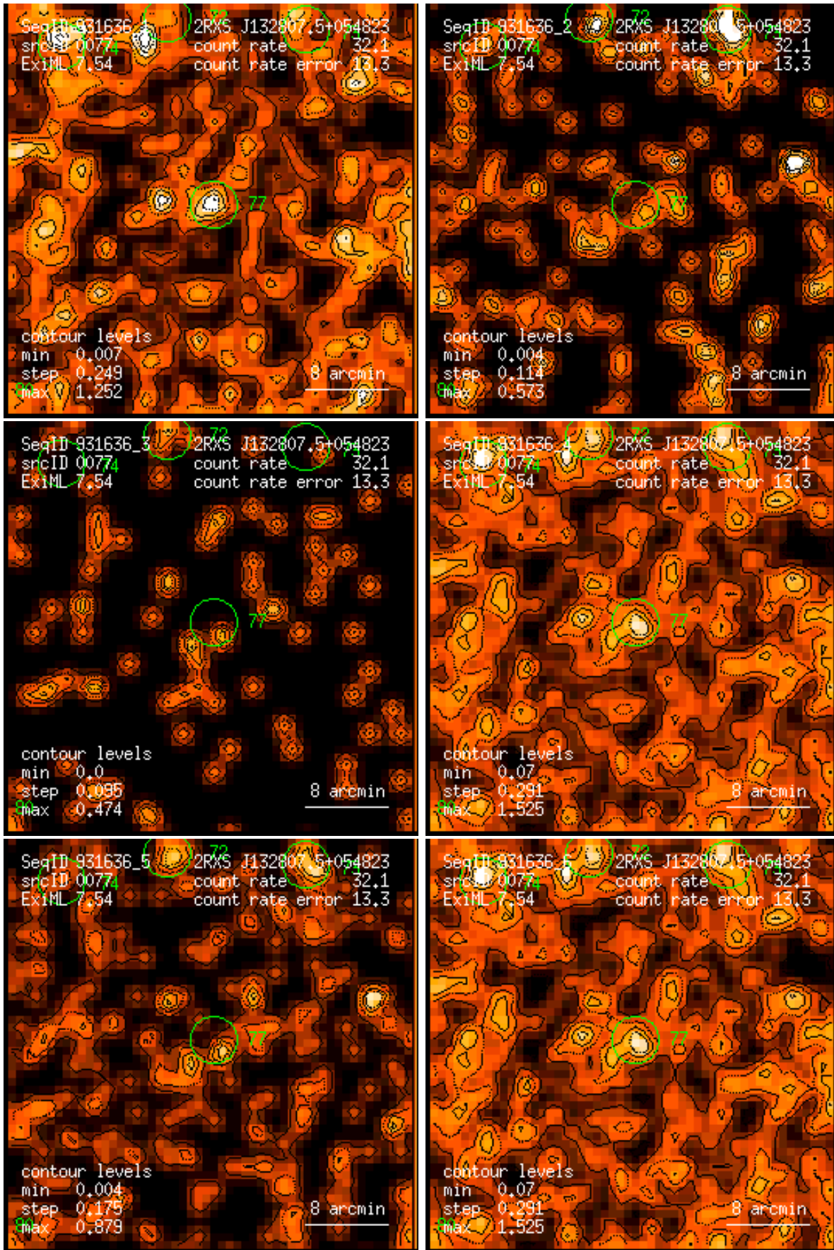
Figure 77: RASS 931636: detection 0077: band rate images, Gaussian filter: (1) PSPC channels 11 – 41, (2) 52 – 90, (3) 91 – 201, (4) 11 – 235, (5) 52 – 201, (6) 11 – 201. Broad band rates in counts/ks. Band rate contour levels in counts/ks/arcmin 2 .
