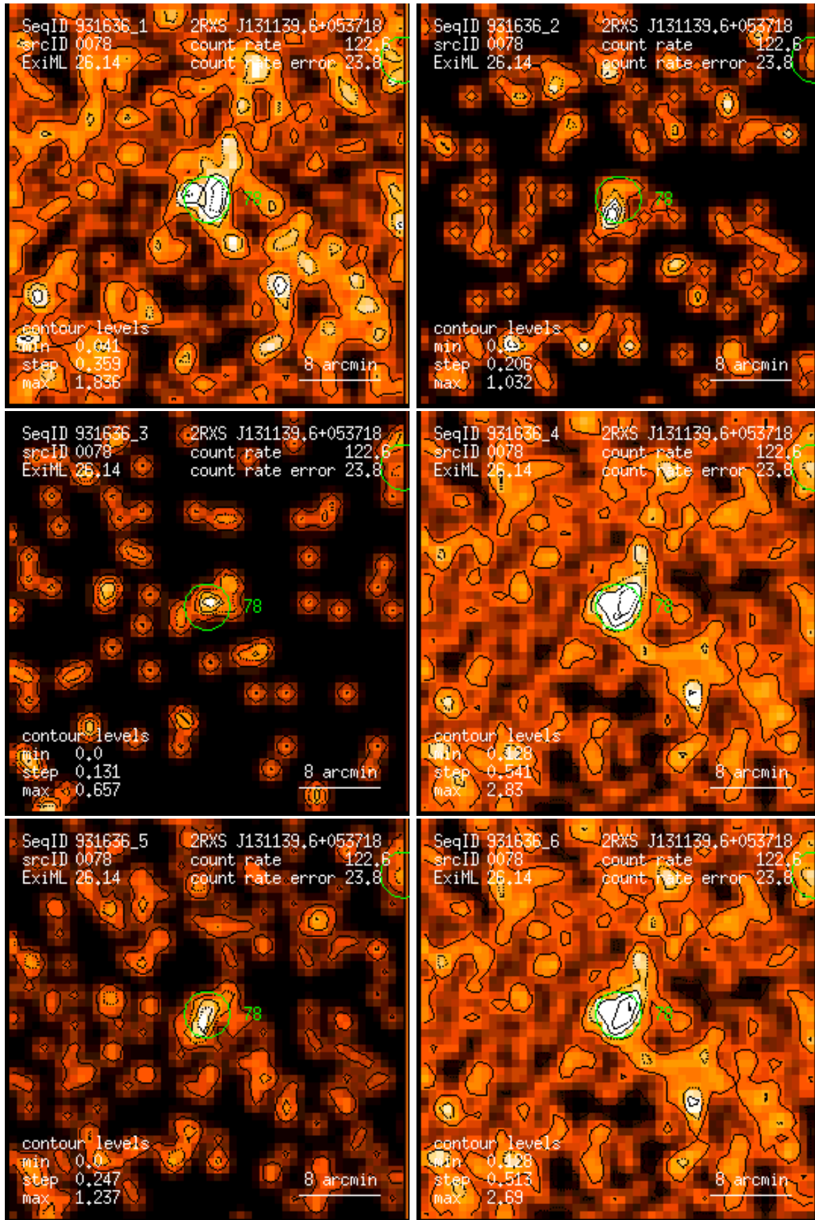
Figure 78: RASS 931636: detection 0078: band rate images, Gaussian filter: (1) PSPC channels 11 – 41, (2) 52 – 90, (3) 91 – 201, (4) 11 – 235, (5) 52 – 201, (6) 11 – 201. Broad band rates in counts/ks. Band rate contour levels in counts/ks/arcmin 2 .
