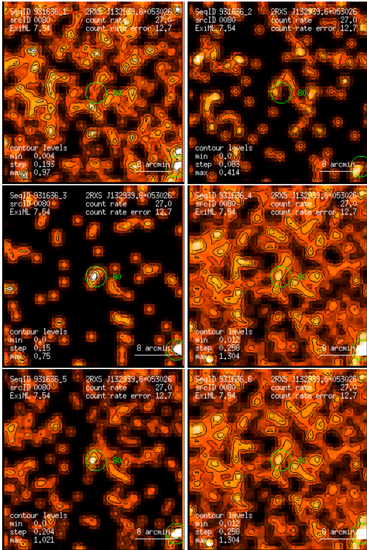
Figure 80: RASS 931636: detection 0080: band rate images, Gaussian filter: (1) PSPC channels 11 – 41, (2) 52 – 90, (3) 91 – 201, (4) 11 – 235, (5) 52 – 201, (6) 11 – 201. Broad band rates in counts/ks. Band rate contour levels in counts/ks/arcmin 2 .
