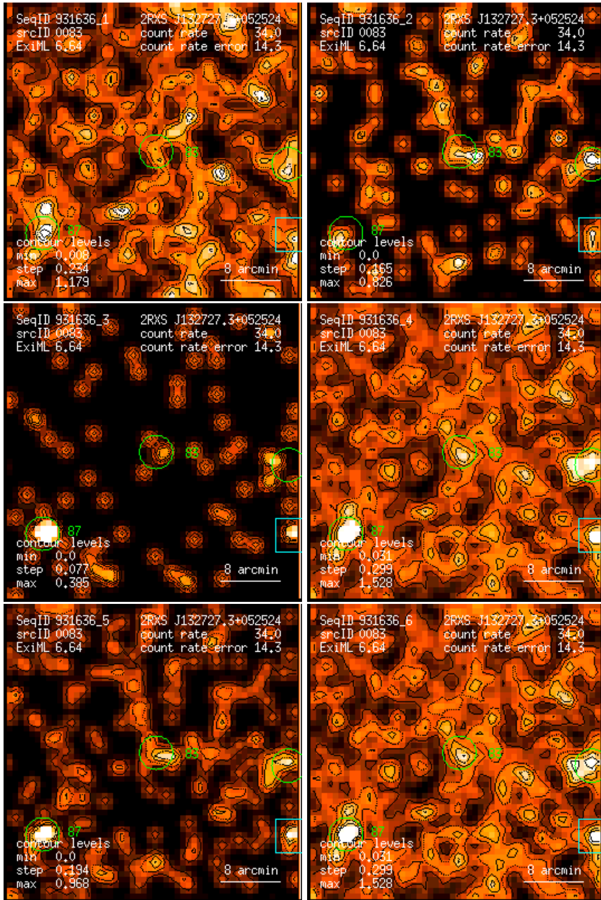
Figure 83: RASS 931636: detection 0083: band rate images, Gaussian filter: (1) PSPC channels 11 – 41, (2) 52 – 90, (3) 91 – 201, (4) 11 – 235, (5) 52 – 201, (6) 11 – 201. Broad band rates in counts/ks. Band rate contour levels in counts/ks/arcmin 2 .
