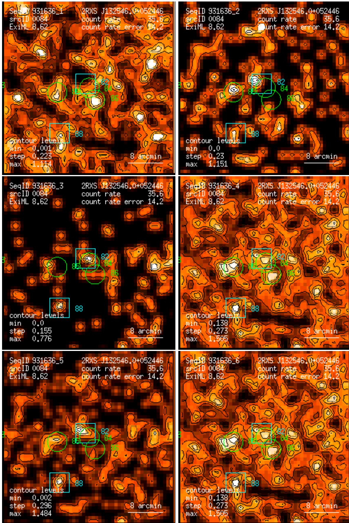
Figure 84: RASS 931636: detection 0084: band rate images, Gaussian filter: (1) PSPC channels 11 – 41, (2) 52 – 90, (3) 91 – 201, (4) 11 – 235, (5) 52 – 201, (6) 11 – 201. Broad band rates in counts/ks. Band rate contour levels in counts/ks/arcmin 2 .
