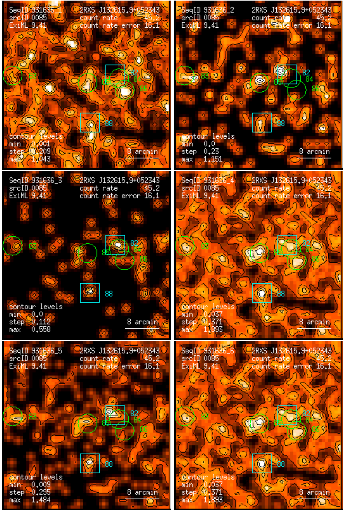
Figure 85: RASS 931636: detection 0085: band rate images, Gaussian filter: (1) PSPC channels 11 – 41, (2) 52 – 90, (3) 91 – 201, (4) 11 – 235, (5) 52 – 201, (6) 11 – 201. Broad band rates in counts/ks. Band rate contour levels in counts/ks/arcmin 2 .
