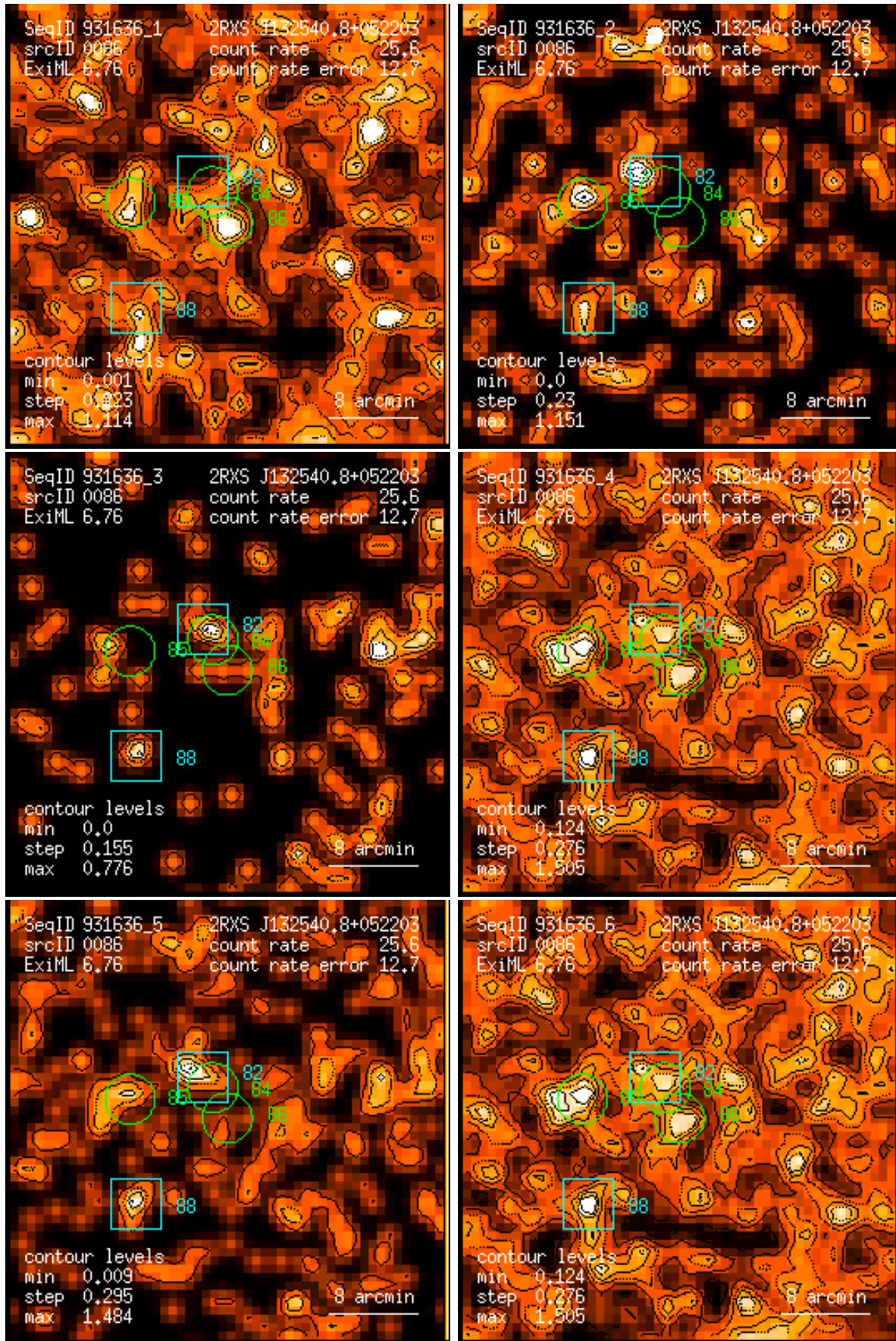
Figure 86: RASS 931636: detection 0086: band rate images, Gaussian filter: (1) PSPC channels 11 – 41, (2) 52 – 90, (3) 91 – 201, (4) 11 – 235, (5) 52 – 201, (6) 11 – 201. Broad band rates in counts/ks. Band rate contour levels in counts/ks/arcmin 2 .
