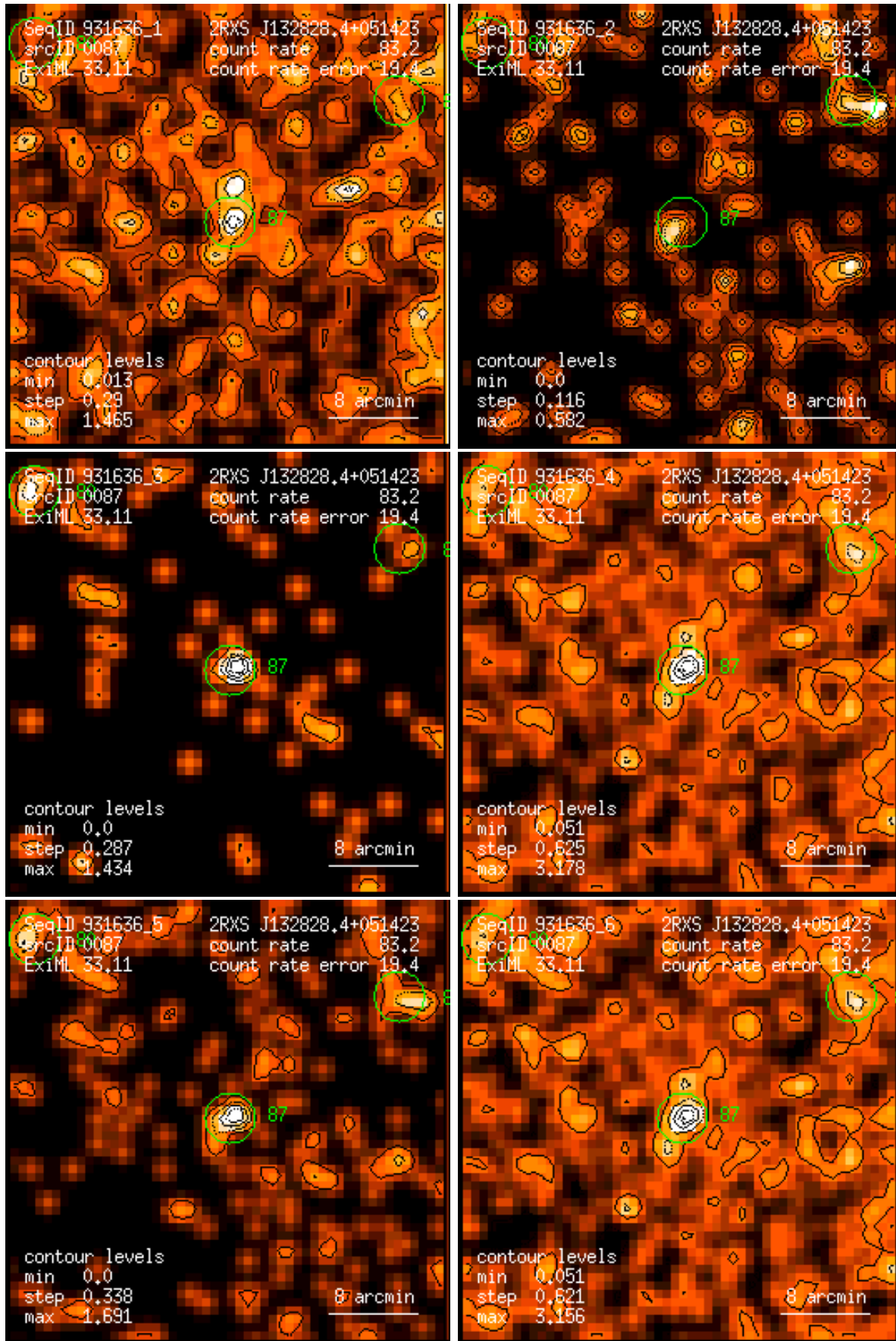
Figure 87: RASS 931636: detection 0087: band rate images, Gaussian filter: (1) PSPC channels 11 – 41, (2) 52 – 90, (3) 91 – 201, (4) 11 – 235, (5) 52 – 201, (6) 11 – 201. Broad band rates in counts/ks. Band rate contour levels in counts/ks/arcmin 2 .
