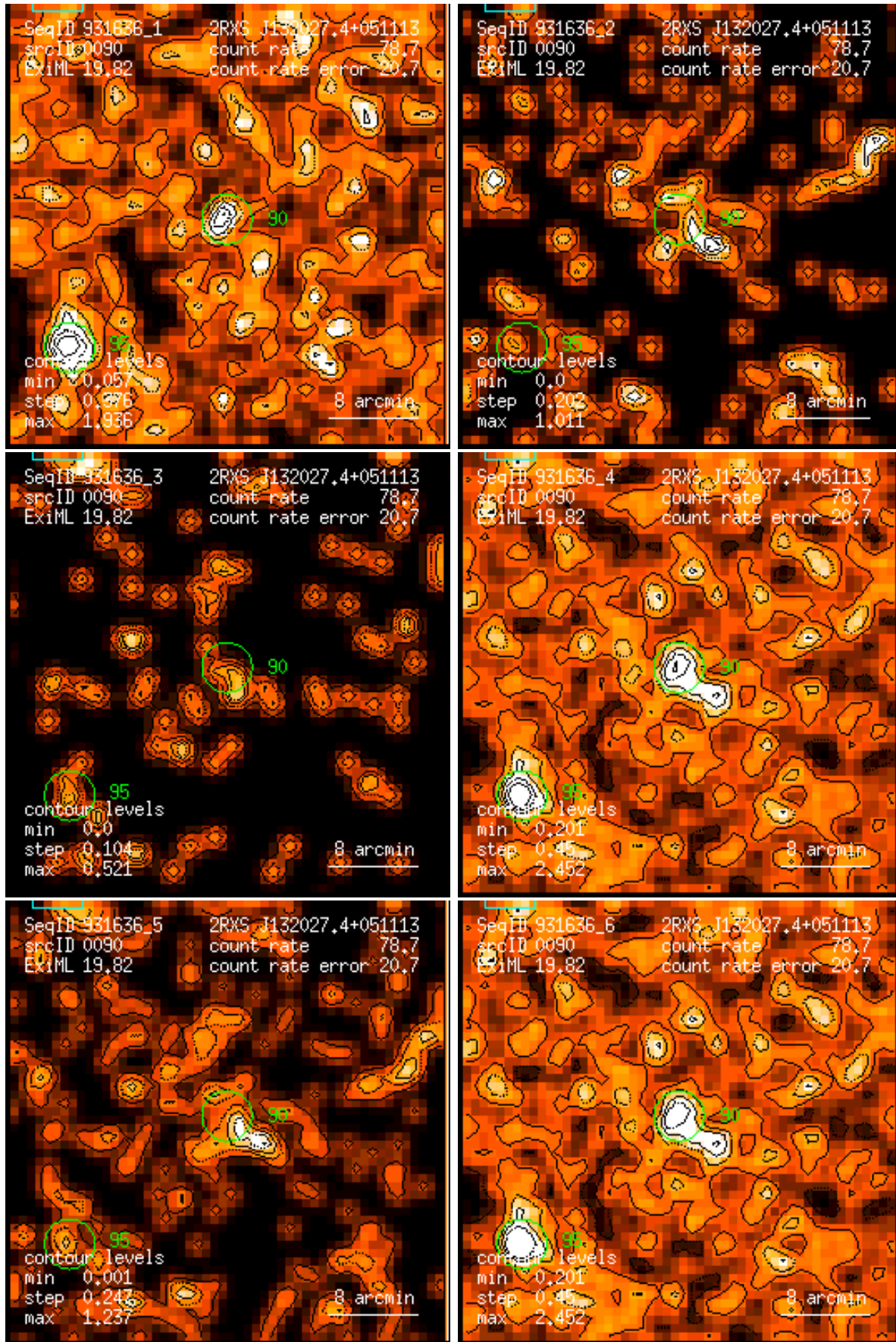
Figure 90: RASS 931636: detection 0090: band rate images, Gaussian filter: (1) PSPC channels 11 – 41, (2) 52 – 90, (3) 91 – 201, (4) 11 – 235, (5) 52 – 201, (6) 11 – 201. Broad band rates in counts/ks. Band rate contour levels in counts/ks/arcmin 2 .
