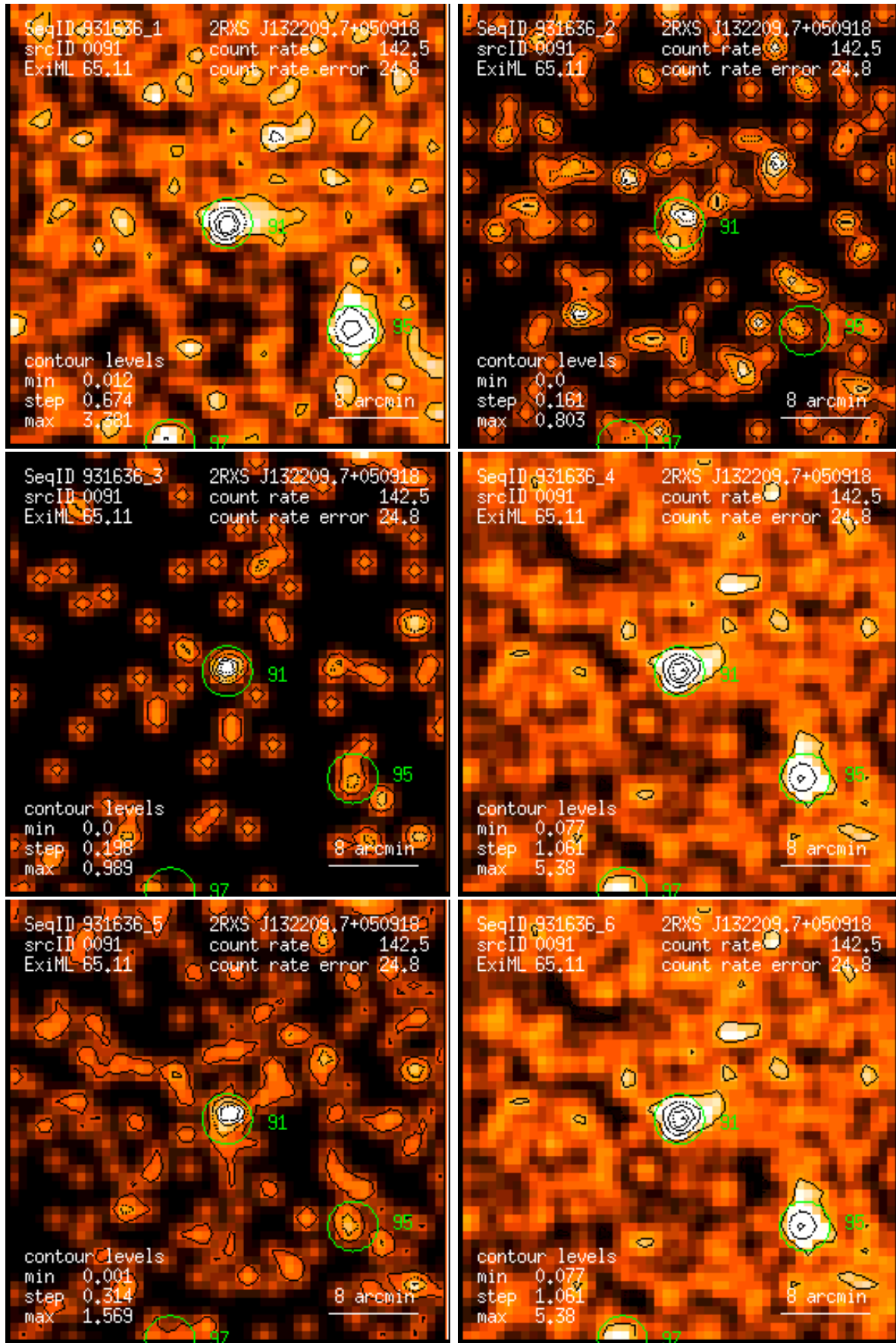
Figure 91: RASS 931636: detection 0091: band rate images, Gaussian filter: (1) PSPC channels 11 – 41, (2) 52 – 90, (3) 91 – 201, (4) 11 – 235, (5) 52 – 201, (6) 11 – 201. Broad band rates in counts/ks. Band rate contour levels in counts/ks/arcmin 2 .
