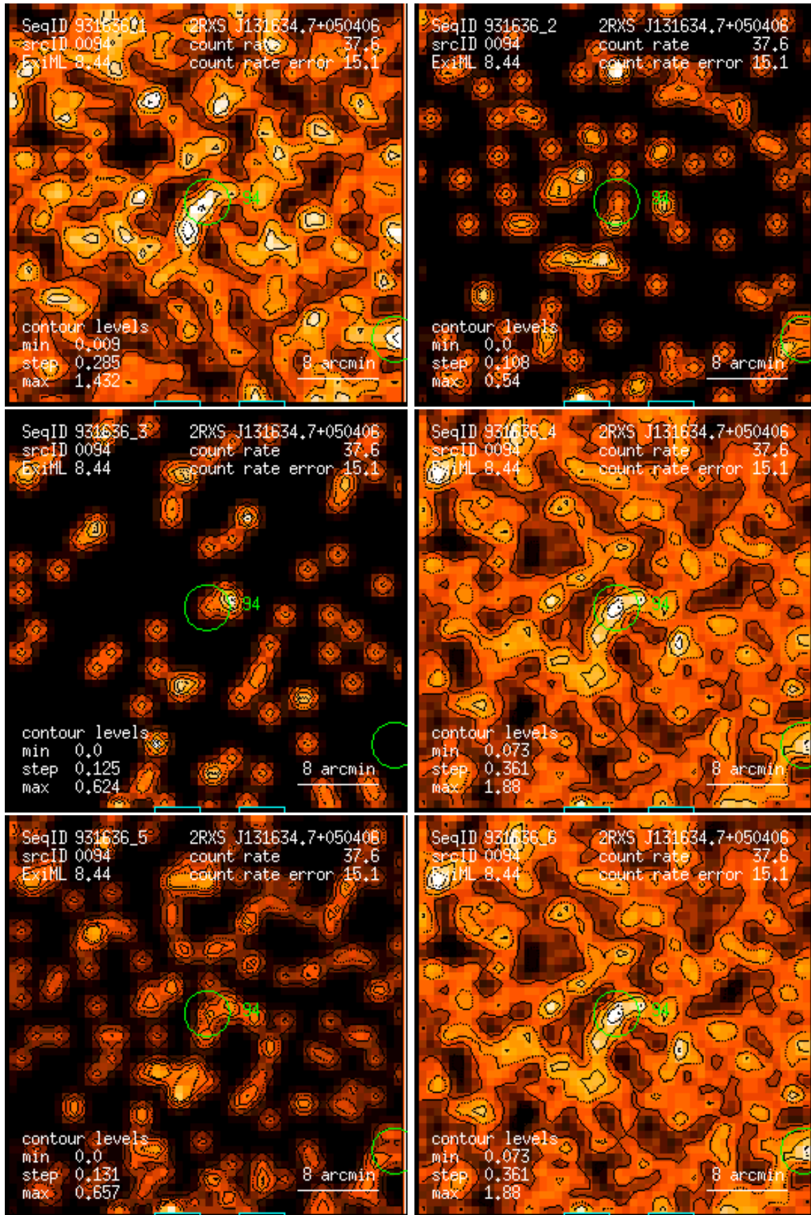
Figure 94: RASS 931636: detection 0094: band rate images, Gaussian filter: (1) PSPC channels 11 – 41, (2) 52 – 90, (3) 91 – 201, (4) 11 – 235, (5) 52 – 201, (6) 11 – 201. Broad band rates in counts/ks. Band rate contour levels in counts/ks/arcmin 2 .
