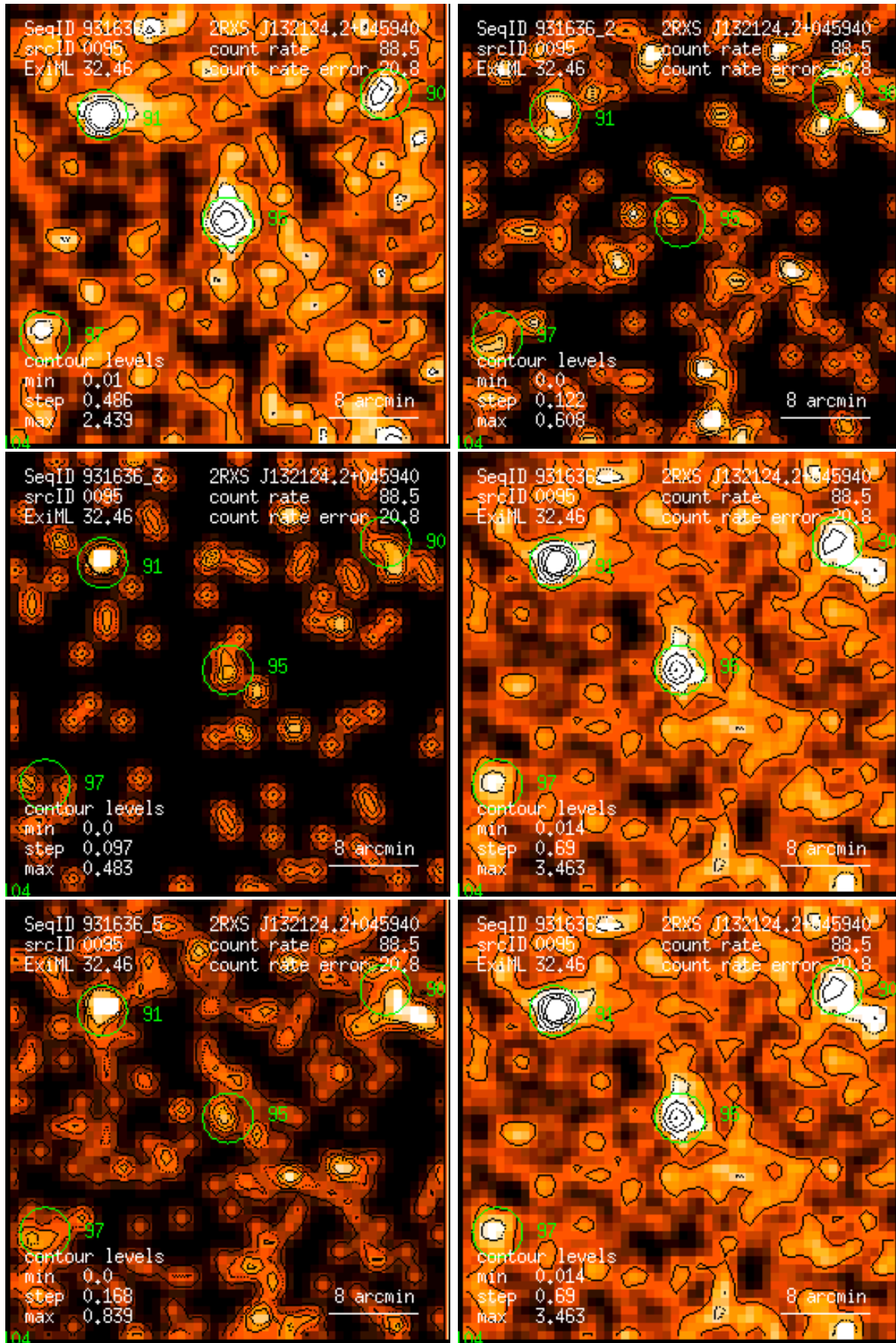
Figure 95: RASS 931636: detection 0095: band rate images, Gaussian filter: (1) PSPC channels 11 – 41, (2) 52 – 90, (3) 91 – 201, (4) 11 – 235, (5) 52 – 201, (6) 11 – 201. Broad band rates in counts/ks. Band rate contour levels in counts/ks/arcmin 2 .
