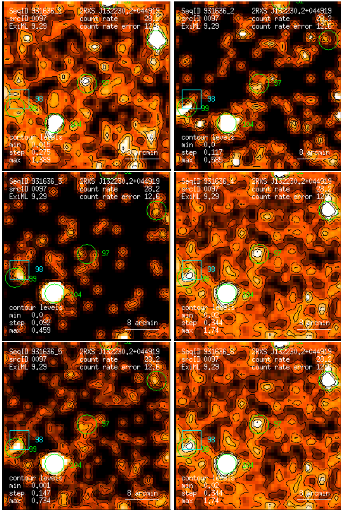
Figure 97: RASS 931636: detection 0097: band rate images, Gaussian filter: (1) PSPC channels 11 – 41, (2) 52 – 90, (3) 91 – 201, (4) 11 – 235, (5) 52 – 201, (6) 11 – 201. Broad band rates in counts/ks. Band rate contour levels in counts/ks/arcmin 2 .
