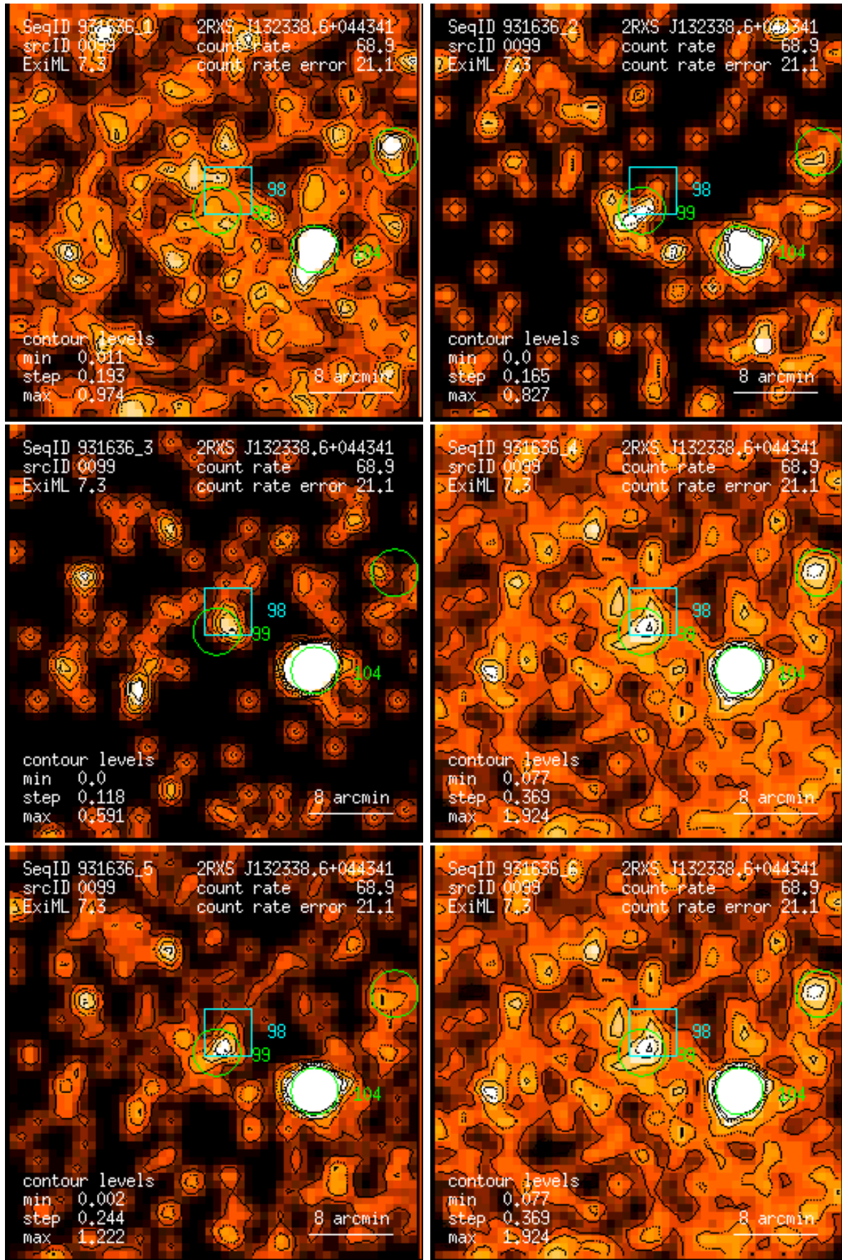
Figure 99: RASS 931636: detection 0099: band rate images, Gaussian filter: (1) PSPC channels 11 – 41, (2) 52 – 90, (3) 91 – 201, (4) 11 – 235, (5) 52 – 201, (6) 11 – 201. Broad band rates in counts/ks. Band rate contour levels in counts/ks/arcmin 2 .
