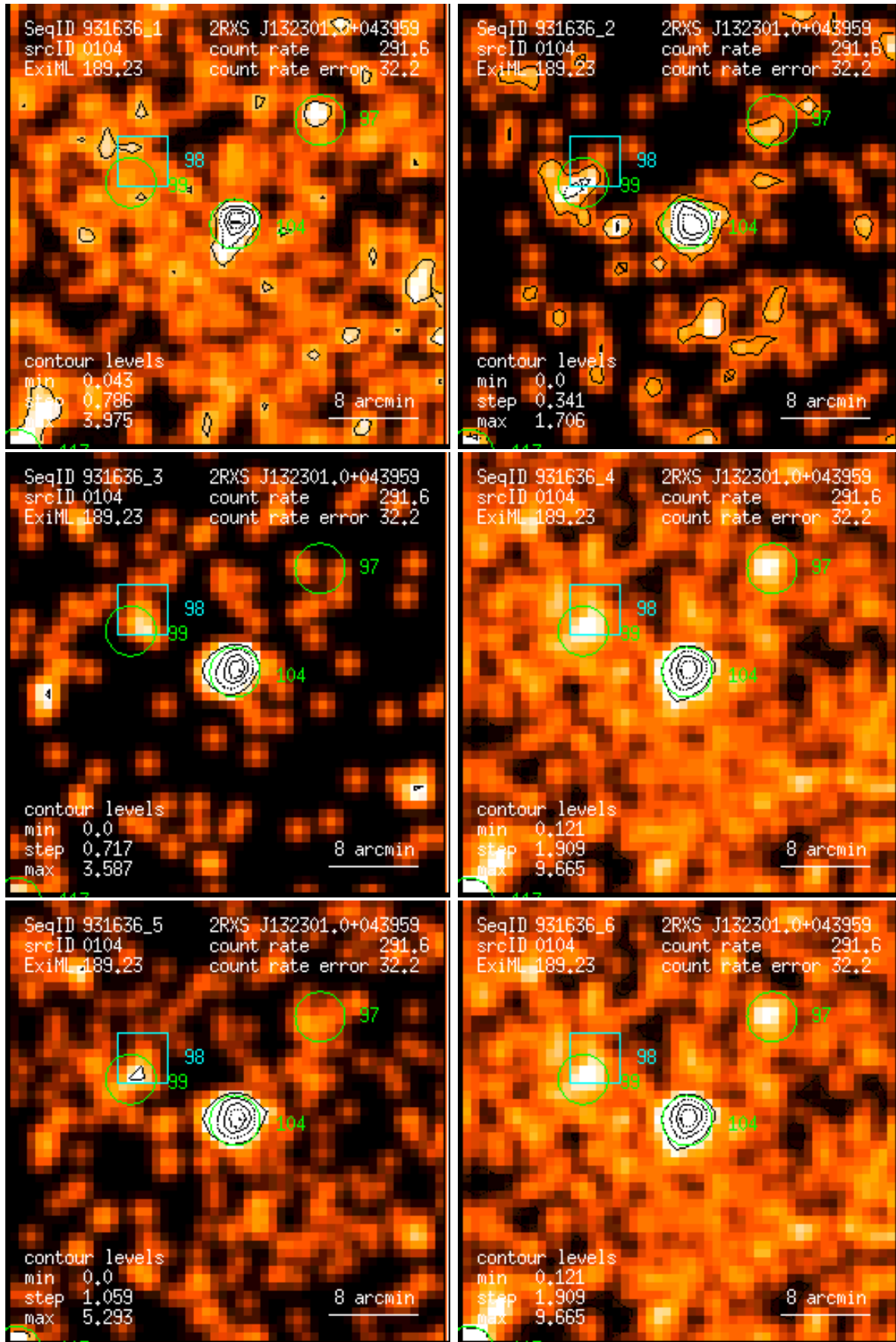
Figure 104: RASS 931636: detection 0104: band rate images, Gaussian filter: (1) PSPC channels 11 – 41, (2) 52 – 90, (3) 91 – 201, (4) 11 – 235, (5) 52 – 201, (6) 11 – 201. Broad band rates in counts/ks. Band rate contour levels in counts/ks/arcmin 2 .
