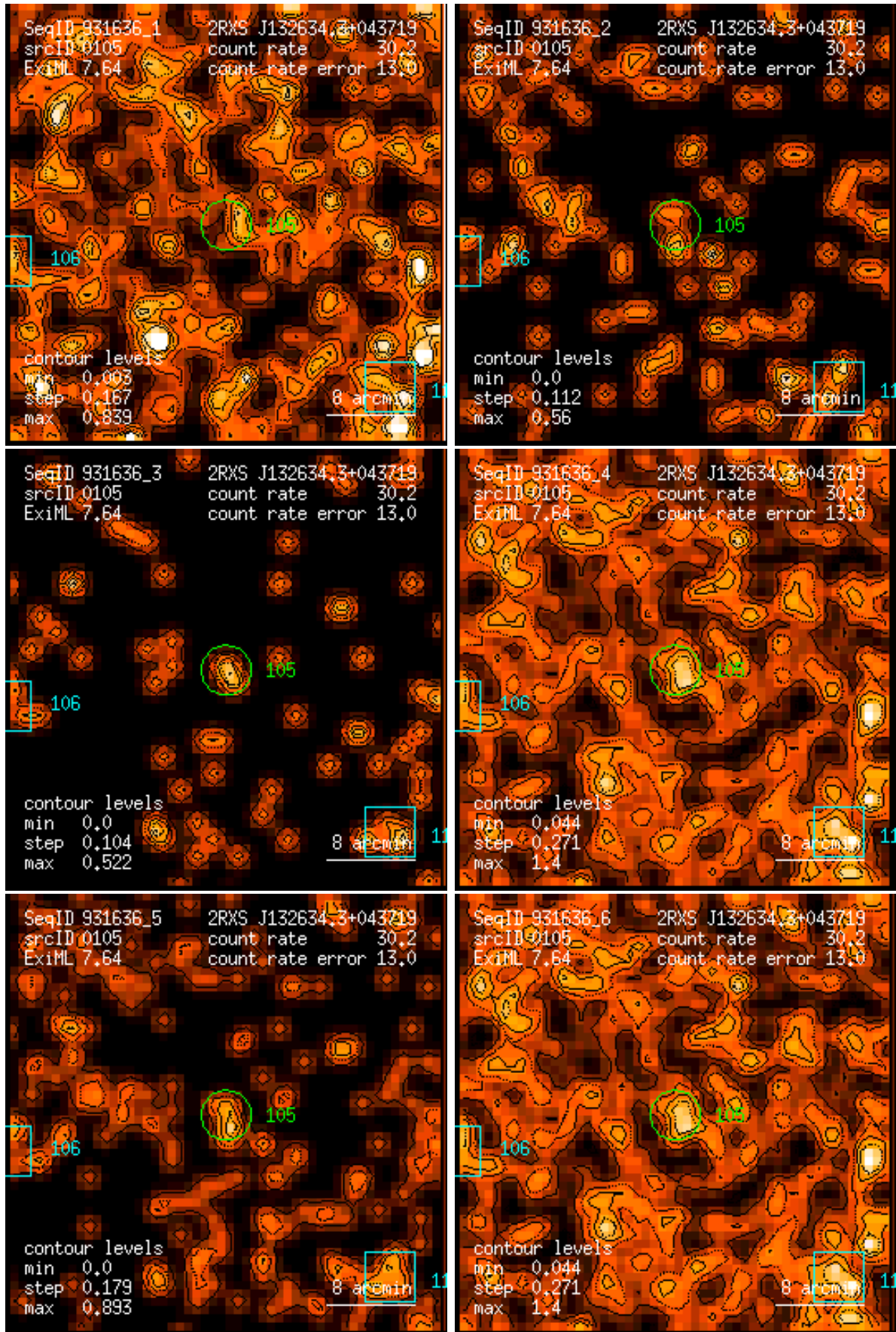
Figure 105: RASS 931636: detection 0105: band rate images, Gaussian filter: (1) PSPC channels 11 – 41, (2) 52 – 90, (3) 91 – 201, (4) 11 – 235, (5) 52 – 201, (6) 11 – 201. Broad band rates in counts/ks. Band rate contour levels in counts/ks/arcmin 2 .
