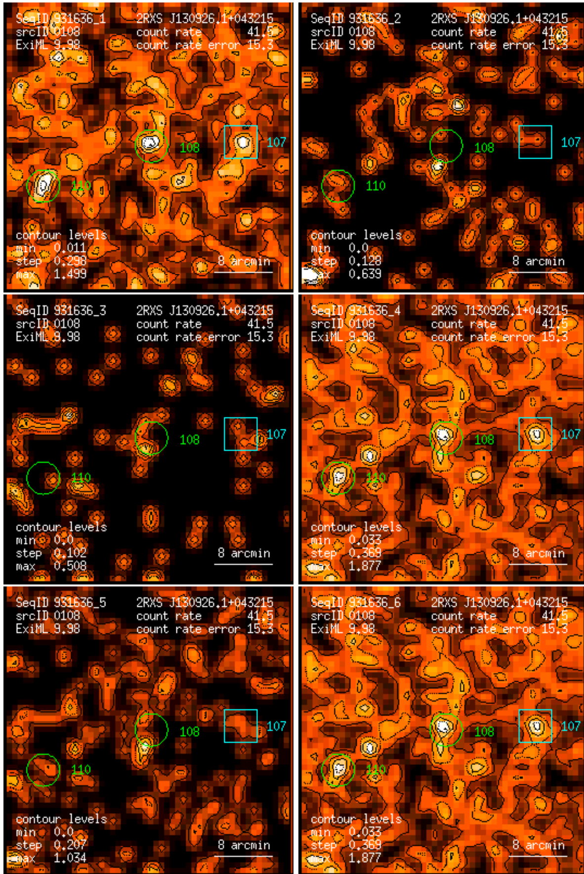
Figure 108: RASS 931636: detection 0108: band rate images, Gaussian filter: (1) PSPC channels 11 – 41, (2) 52 – 90, (3) 91 – 201, (4) 11 – 235, (5) 52 – 201, (6) 11 – 201. Broad band rates in counts/ks. Band rate contour levels in counts/ks/arcmin 2 .
