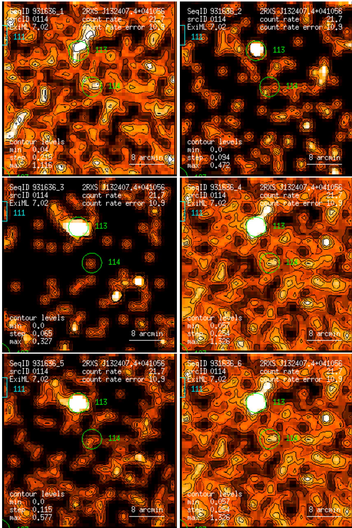
Figure 114: RASS 931636: detection 0114: band rate images, Gaussian filter: (1) PSPC channels 11 – 41, (2) 52 – 90, (3) 91 – 201, (4) 11 – 235, (5) 52 – 201, (6) 11 – 201. Broad band rates in counts/ks. Band rate contour levels in counts/ks/arcmin 2 .
