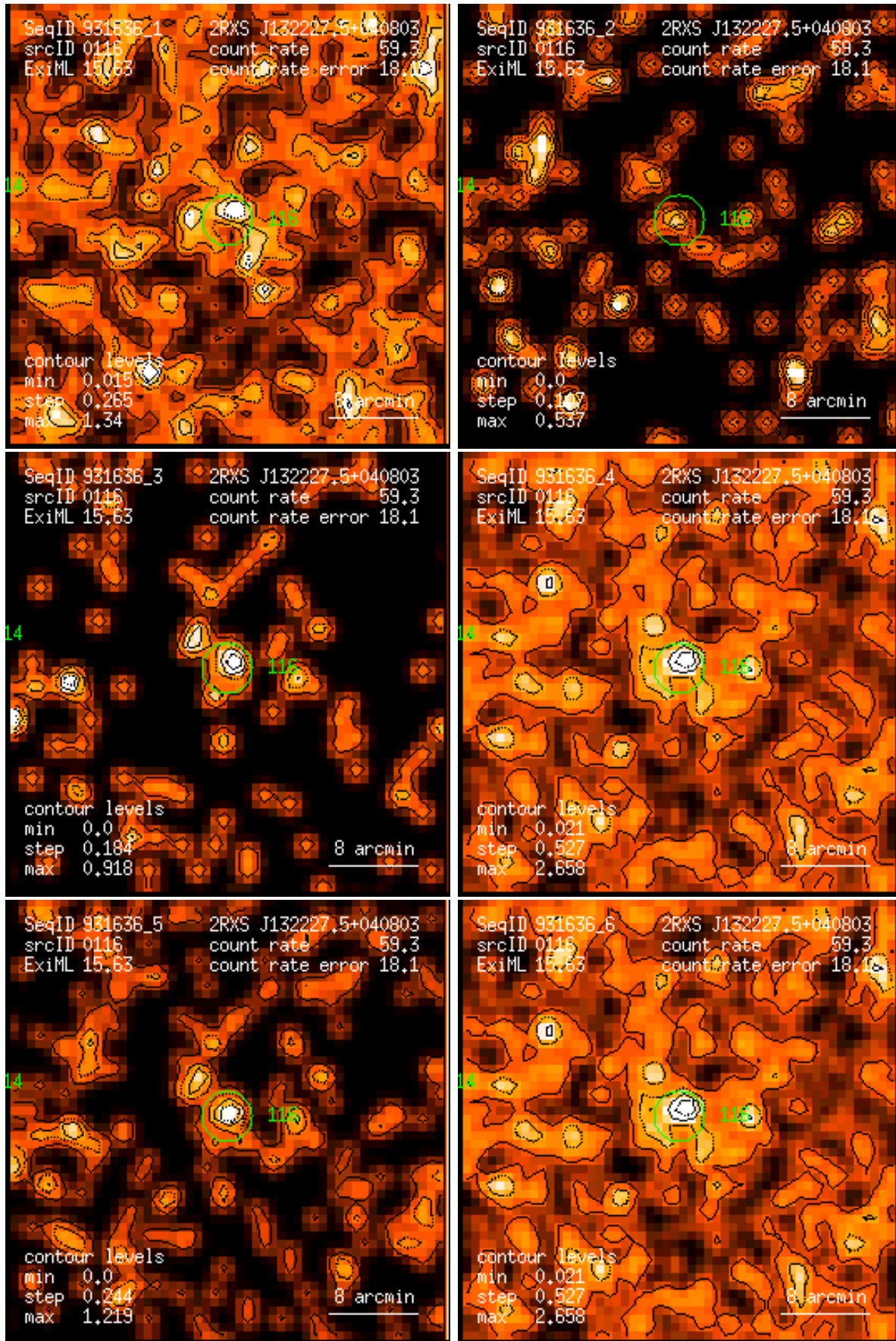
Figure 116: RASS 931636: detection 0116: band rate images, Gaussian filter: (1) PSPC channels 11 – 41, (2) 52 – 90, (3) 91 – 201, (4) 11 – 235, (5) 52 – 201, (6) 11 – 201. Broad band rates in counts/ks. Band rate contour levels in counts/ks/arcmin 2 .
