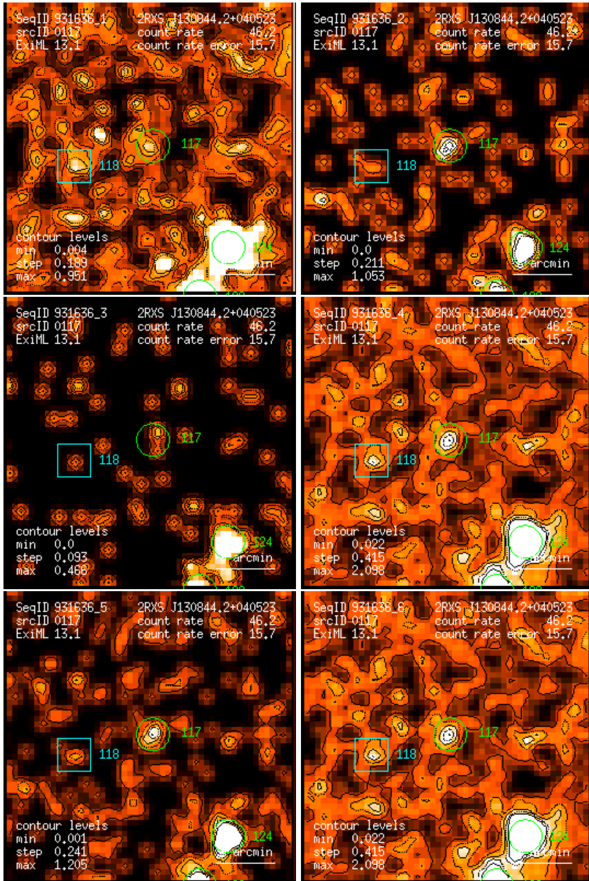
Figure 117: RASS 931636: detection 0117: band rate images, Gaussian filter: (1) PSPC channels 11 – 41, (2) 52 – 90, (3) 91 – 201, (4) 11 – 235, (5) 52 – 201, (6) 11 – 201. Broad band rates in counts/ks. Band rate contour levels in counts/ks/arcmin 2 .
