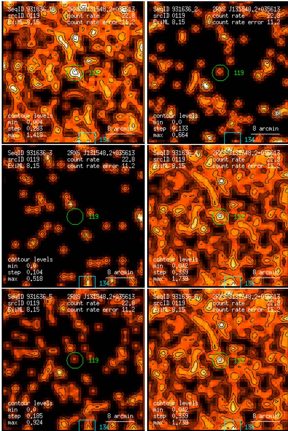
Figure 119: RASS 931636: detection 0119: band rate images, Gaussian filter: (1) PSPC channels 11 – 41, (2) 52 – 90, (3) 91 – 201, (4) 11 – 235, (5) 52 – 201, (6) 11 – 201. Broad band rates in counts/ks. Band rate contour levels in counts/ks/arcmin 2 .
