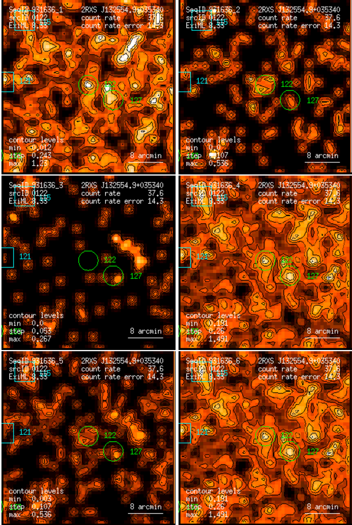
Figure 122: RASS 931636: detection 0122: band rate images, Gaussian filter: (1) PSPC channels 11 – 41, (2) 52 – 90, (3) 91 – 201, (4) 11 – 235, (5) 52 – 201, (6) 11 – 201. Broad band rates in counts/ks. Band rate contour levels in counts/ks/arcmin 2 .
