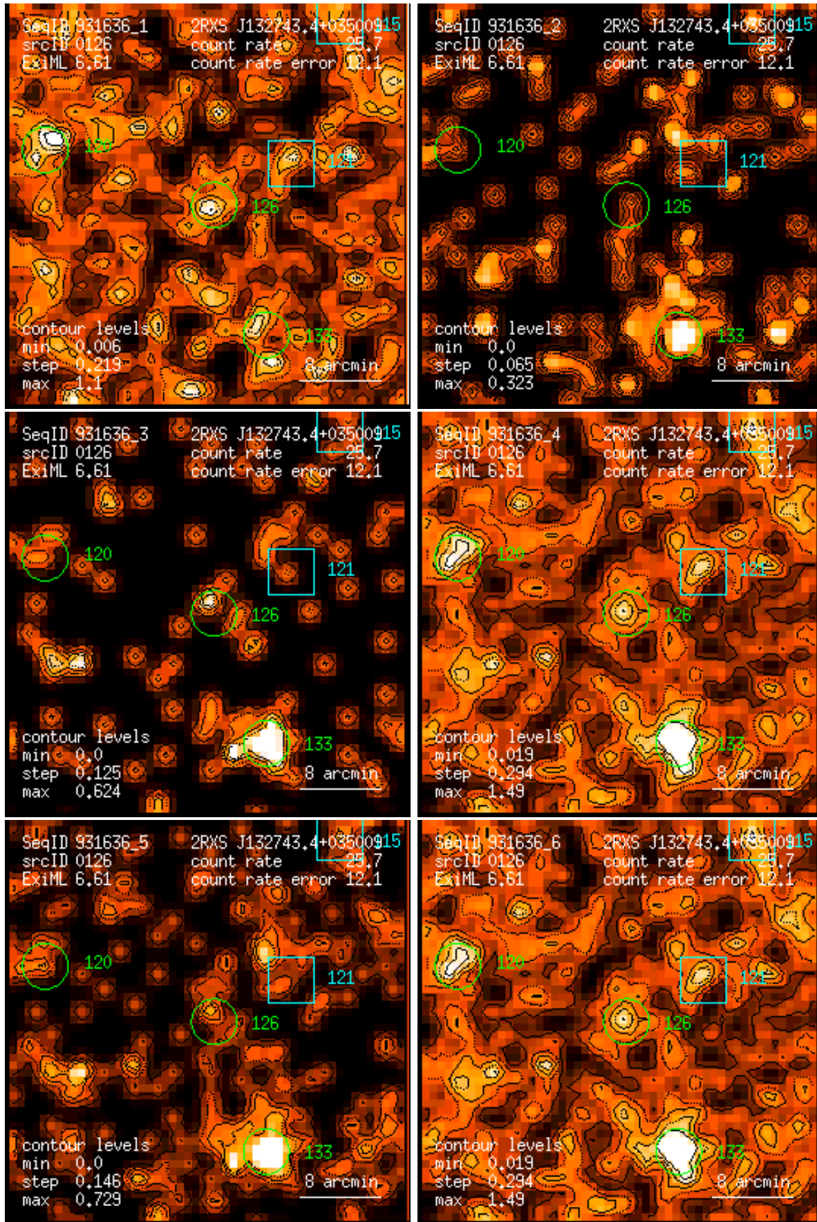
Figure 126: RASS 931636: detection 0126: band rate images, Gaussian filter: (1) PSPC channels 11 – 41, (2) 52 – 90, (3) 91 – 201, (4) 11 – 235, (5) 52 – 201, (6) 11 – 201. Broad band rates in counts/ks. Band rate contour levels in counts/ks/arcmin 2 .
