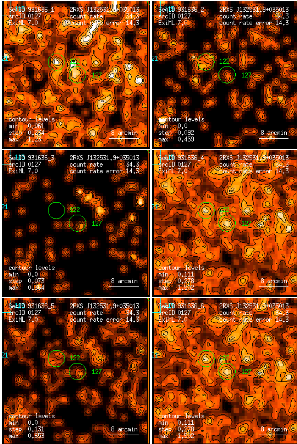
Figure 127: RASS 931636: detection 0127: band rate images, Gaussian filter: (1) PSPC channels 11 – 41, (2) 52 – 90, (3) 91 – 201, (4) 11 – 235, (5) 52 – 201, (6) 11 – 201. Broad band rates in counts/ks. Band rate contour levels in counts/ks/arcmin 2 .
