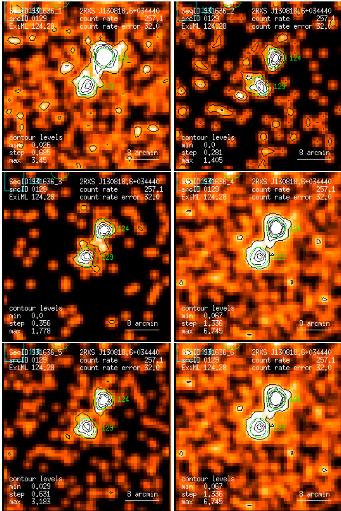
Figure 129: RASS 931636: detection 0129: band rate images, Gaussian filter: (1) PSPC channels 11 – 41, (2) 52 – 90, (3) 91 – 201, (4) 11 – 235, (5) 52 – 201, (6) 11 – 201. Broad band rates in counts/ks. Band rate contour levels in counts/ks/arcmin 2 .
