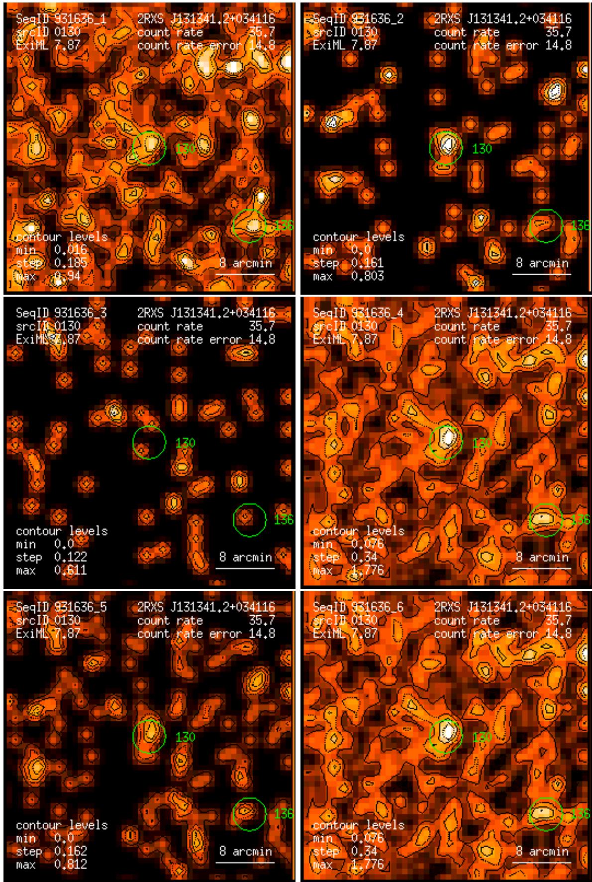
Figure 130: RASS 931636: detection 0130: band rate images, Gaussian filter: (1) PSPC channels 11 – 41, (2) 52 – 90, (3) 91 – 201, (4) 11 – 235, (5) 52 – 201, (6) 11 – 201. Broad band rates in counts/ks. Band rate contour levels in counts/ks/arcmin 2 .
