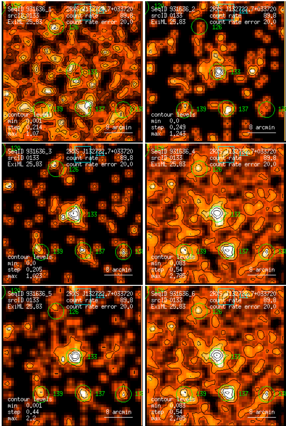
Figure 133: RASS 931636: detection 0133: band rate images, Gaussian filter: (1) PSPC channels 11 – 41, (2) 52 – 90, (3) 91 – 201, (4) 11 – 235, (5) 52 – 201, (6) 11 – 201. Broad band rates in counts/ks. Band rate contour levels in counts/ks/arcmin 2 .
