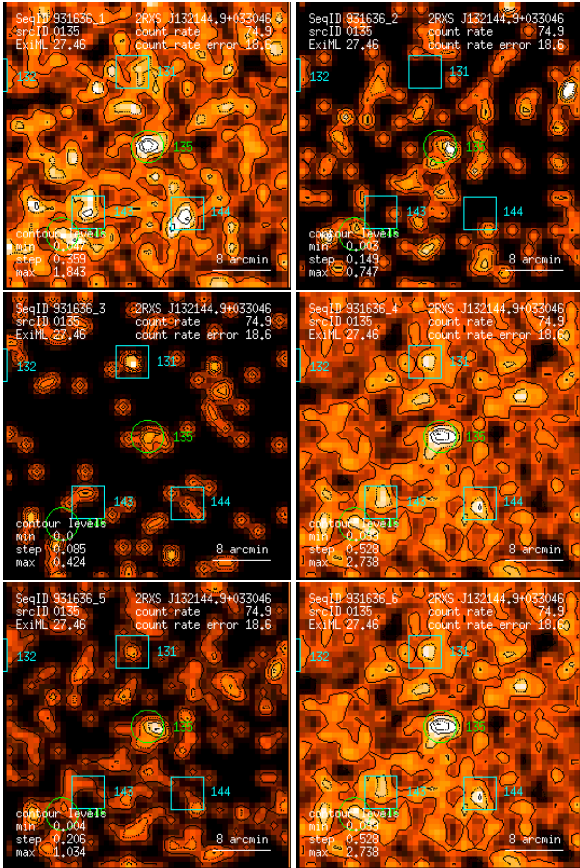
Figure 135: RASS 931636: detection 0135: band rate images, Gaussian filter: (1) PSPC channels 11 – 41, (2) 52 – 90, (3) 91 – 201, (4) 11 – 235, (5) 52 – 201, (6) 11 – 201. Broad band rates in counts/ks. Band rate contour levels in counts/ks/arcmin 2 .
