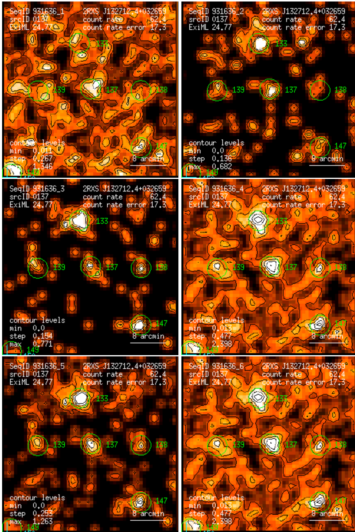
Figure 137: RASS 931636: detection 0137: band rate images, Gaussian filter: (1) PSPC channels 11 – 41, (2) 52 – 90, (3) 91 – 201, (4) 11 – 235, (5) 52 – 201, (6) 11 – 201. Broad band rates in counts/ks. Band rate contour levels in counts/ks/arcmin 2 .
