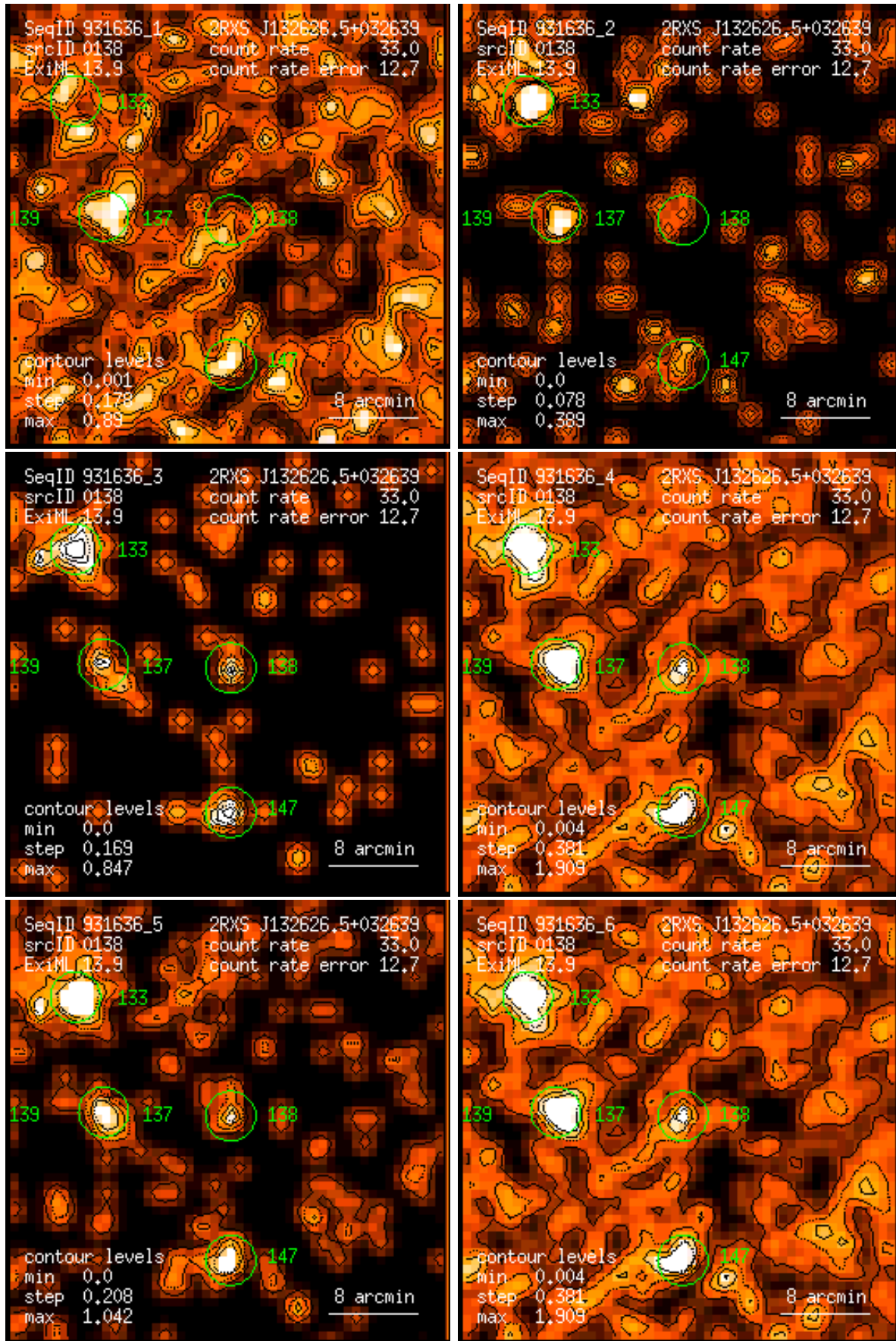
Figure 138: RASS 931636: detection 0138: band rate images, Gaussian filter: (1) PSPC channels 11 – 41, (2) 52 – 90, (3) 91 – 201, (4) 11 – 235, (5) 52 – 201, (6) 11 – 201. Broad band rates in counts/ks. Band rate contour levels in counts/ks/arcmin 2 .
