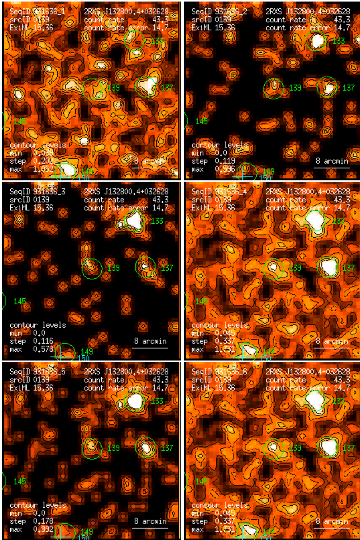
Figure 139: RASS 931636: detection 0139: band rate images, Gaussian filter: (1) PSPC channels 11 – 41, (2) 52 – 90, (3) 91 – 201, (4) 11 – 235, (5) 52 – 201, (6) 11 – 201. Broad band rates in counts/ks. Band rate contour levels in counts/ks/arcmin 2 .
