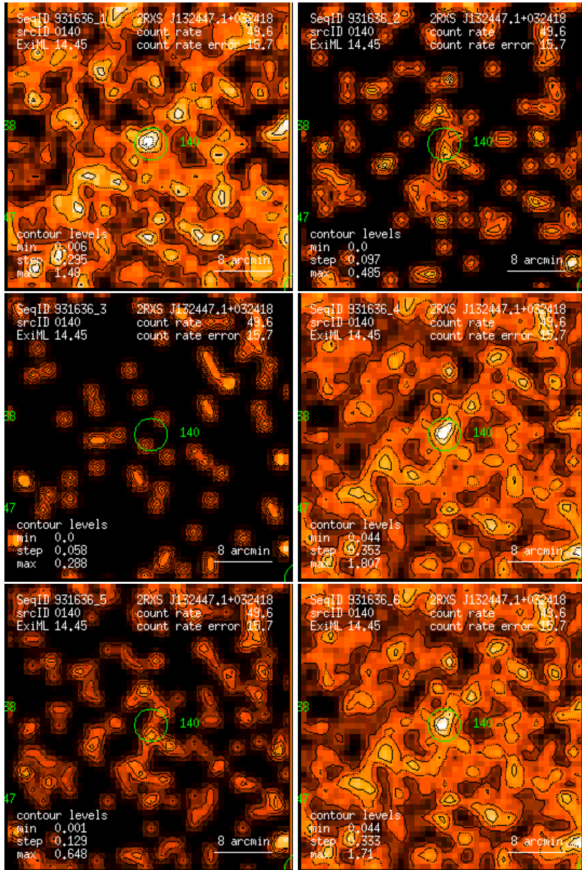
Figure 140: RASS 931636: detection 0140: band rate images, Gaussian filter: (1) PSPC channels 11 – 41, (2) 52 – 90, (3) 91 – 201, (4) 11 – 235, (5) 52 – 201, (6) 11 – 201. Broad band rates in counts/ks. Band rate contour levels in counts/ks/arcmin 2 .
