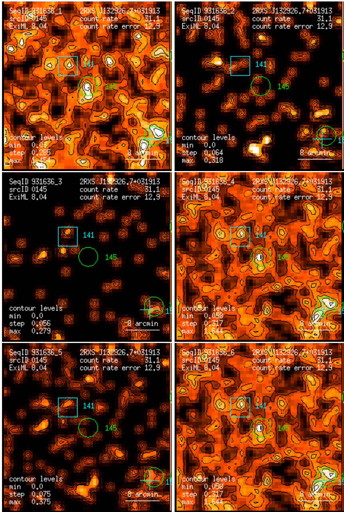
Figure 145: RASS 931636: detection 0145: band rate images, Gaussian filter: (1) PSPC channels 11 – 41, (2) 52 – 90, (3) 91 – 201, (4) 11 – 235, (5) 52 – 201, (6) 11 – 201. Broad band rates in counts/ks. Band rate contour levels in counts/ks/arcmin 2 .
