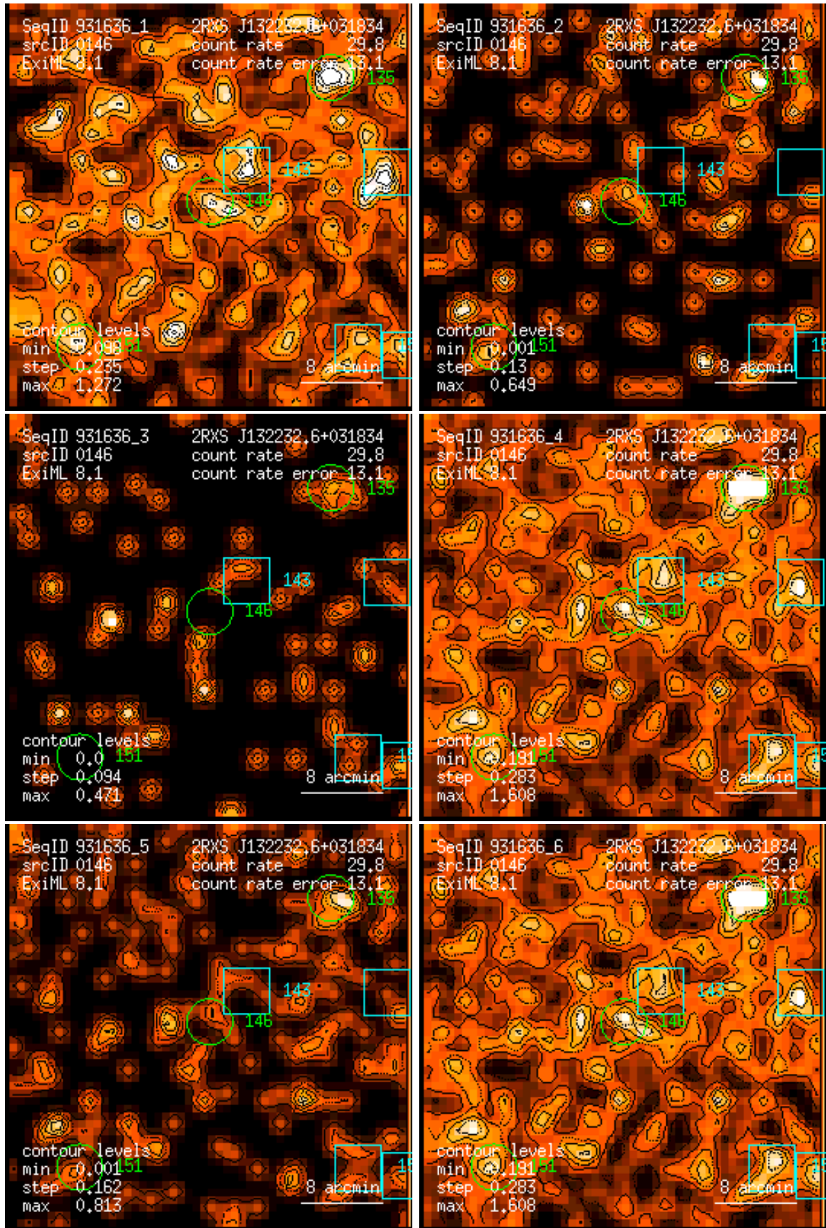
Figure 146: RASS 931636: detection 0146: band rate images, Gaussian filter: (1) PSPC channels 11 – 41, (2) 52 – 90, (3) 91 – 201, (4) 11 – 235, (5) 52 – 201, (6) 11 – 201. Broad band rates in counts/ks. Band rate contour levels in counts/ks/arcmin 2 .
